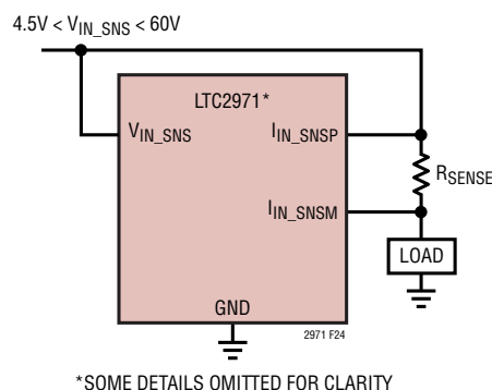
Figure 24. Measuring Input Current
