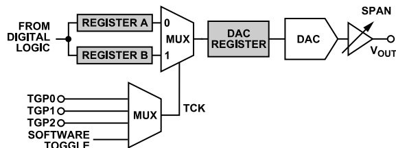
Figure 53. Toggle Operation
