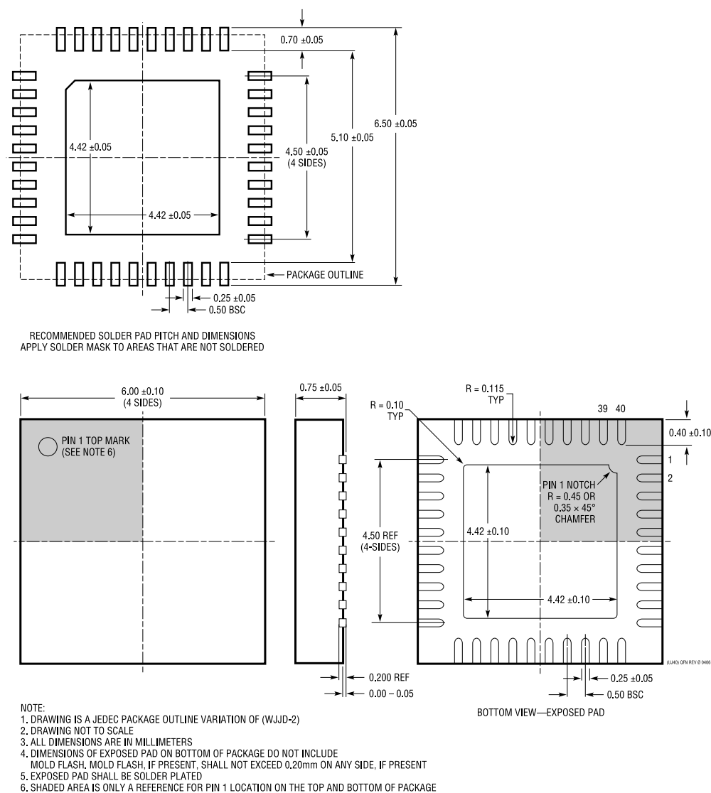
Figure 61. 40-Lead Lead Frame Chip Scale Package [LFCSP] 6 mm × 6 mm Body and 0.75 mm Package Height 05-08-1728 Dimensions shown in millimeters
