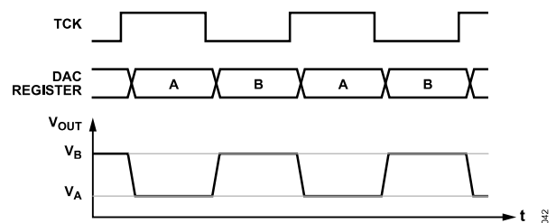
Figure 54. TCK Timing
