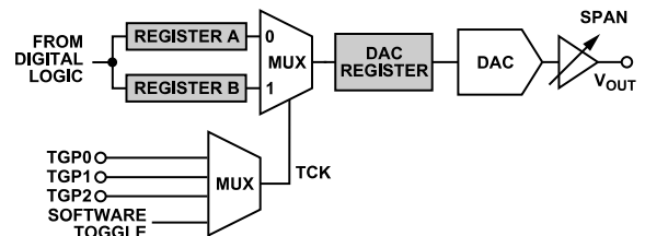
Figure 53. Toggle Operation
