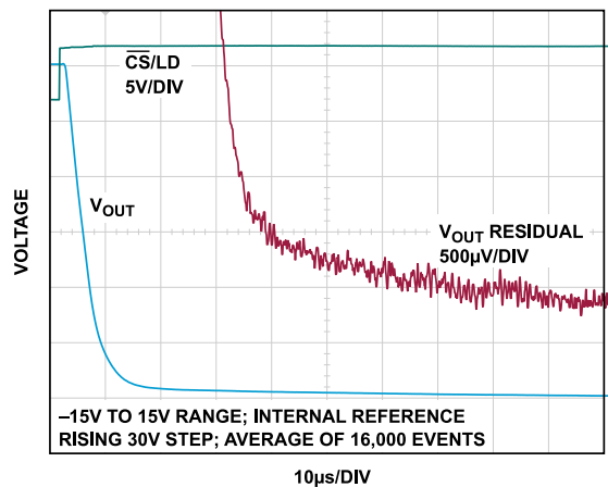
Figure 43. Settling Time, 30 V (Falling)
