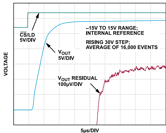
Figure 42. Settling Time, 30 V
