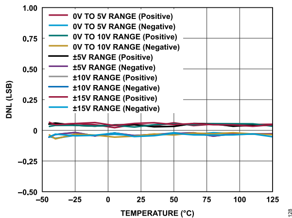
Figure 29. LTC2686-16 DNL vs. Temperature
