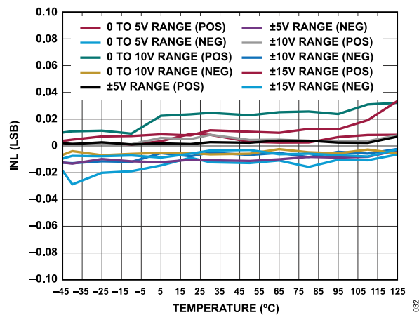
Figure 32. LTC2686-12 INL vs. Temperature
