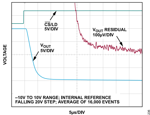
Figure 41. Settling Time, 20 V (Falling)
