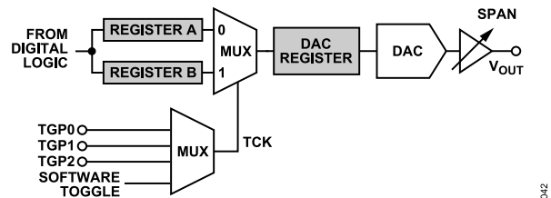
Figure 53. Toggle Operation
