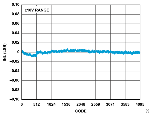
Figure 30. LTC2686-12 INL vs. Code
