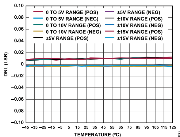
Figure 33. LTC2686-12 DNL vs. Temperature
