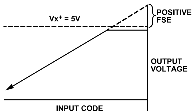
Figure 60. Effect of Negative Offset for Codes Near Zero Scale
