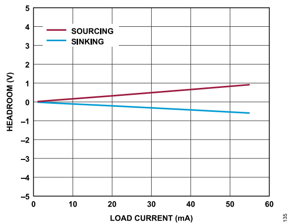
Figure 44. V_{x^+}/V^- Unipolar Headroom vs. Output Load Current
