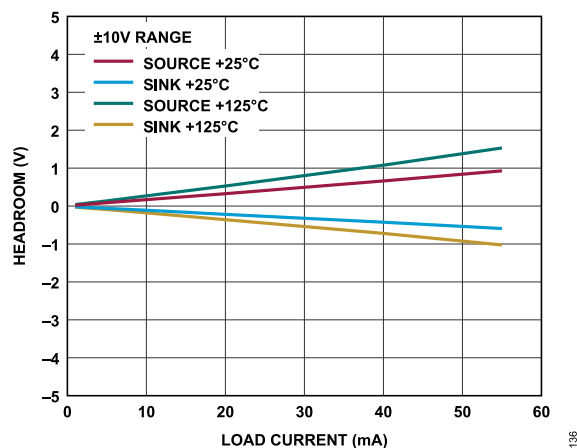
Figure 45. V_{x^+}/V^- Bipolar Headroom vs. Output Load Current
