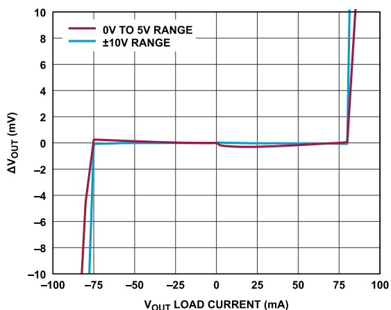
Figure 19. ΔV OUT vs. V OUT Load Current
