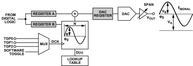
Figure 55. Dither Signal Operation
