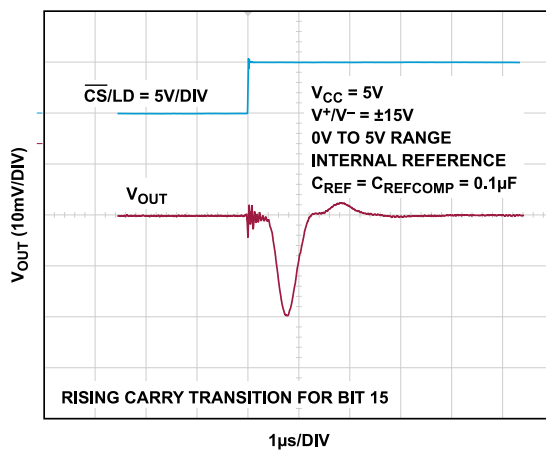
Figure 16. Glitch Impulse
