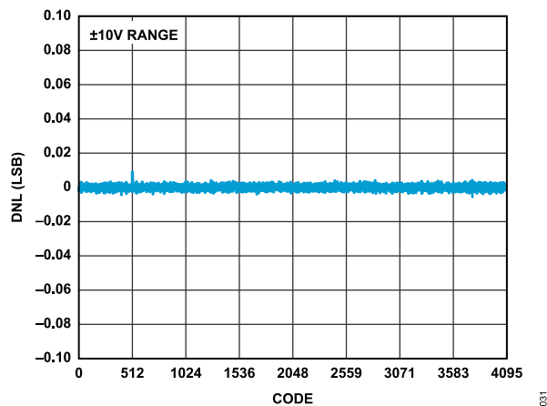
Figure 31. LTC2686-12 DNL vs. Code
