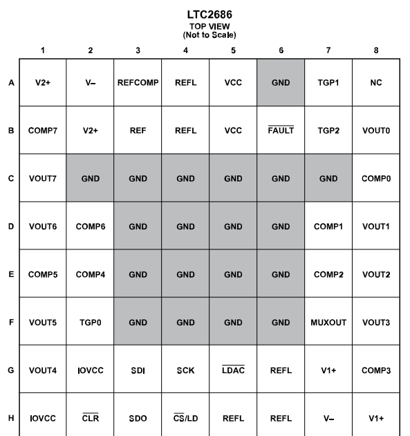
Figure 4. WLCSP Pin Configuration
