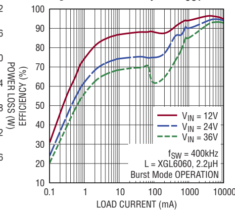
Light Load Efficiency at 5V OUT
