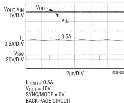
Switching Waveforms, Frequency Foldback when VIN is close to VOUT
