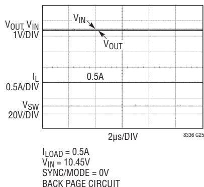
Waveforms, PassThru Mode Operation
