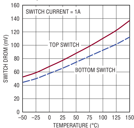
Power Switch Voltage Drop vs Temperature
