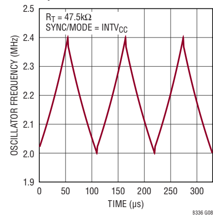
Oscillator Frequency with Spread Spectrum Modulation
