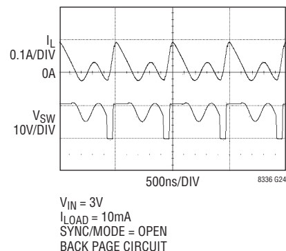
Switching Waveforms, Discontinuous Pulse-Skipping Mode
