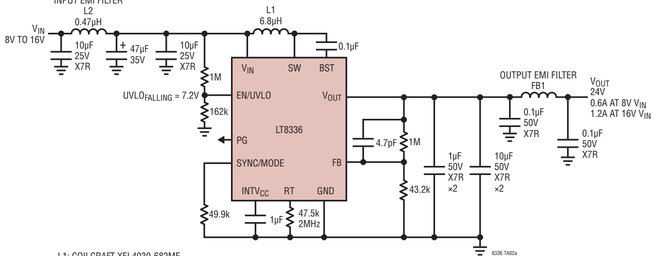
Low I_Q , Low EMI, 24V Output Boost Converter with SSFM*
