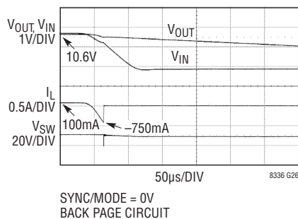
Waveforms, Reverse Current Protection in PassThru Mode
