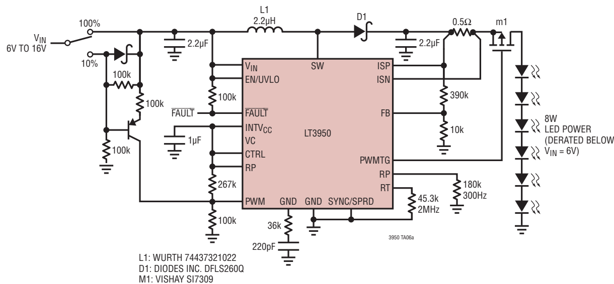
2MHz, 8W and 0.8W Input Boost LED Driver
