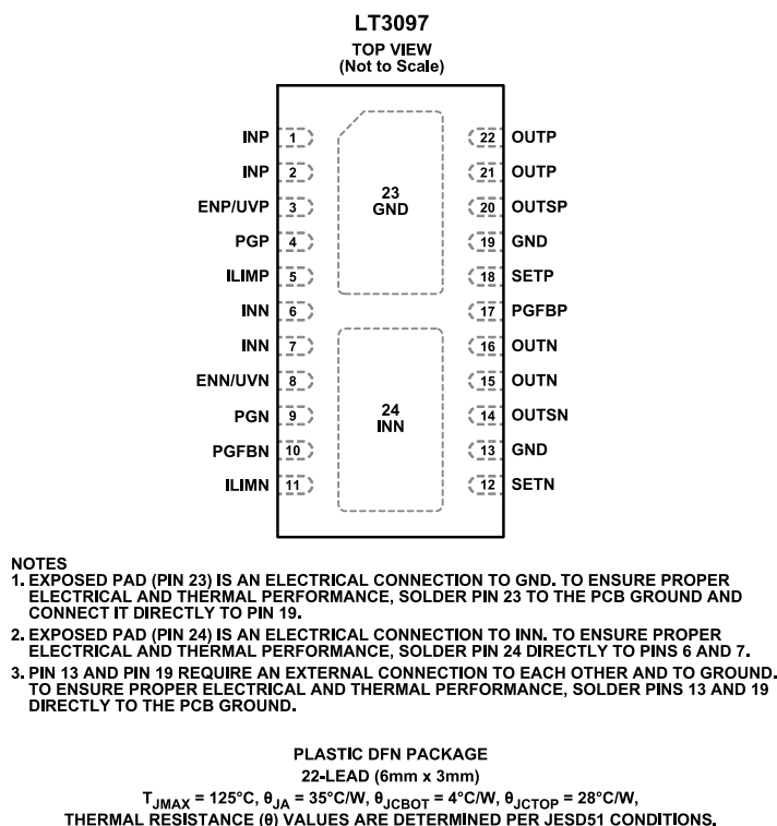
Figure 3. Pin Configuration
