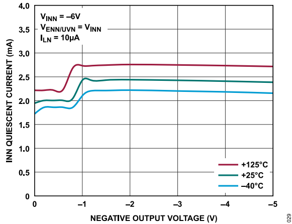
Figure 29. INN Quiescent Current vs. Negative Output Voltage
