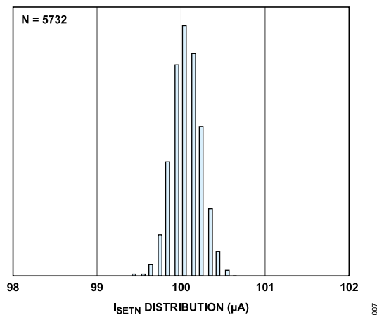
Figure 7. I_{SETN} Distribution
