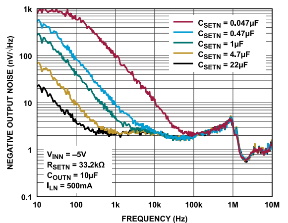
Figure 99. Negative Output Noise vs. Frequency ( C_{SETN} Steps)
