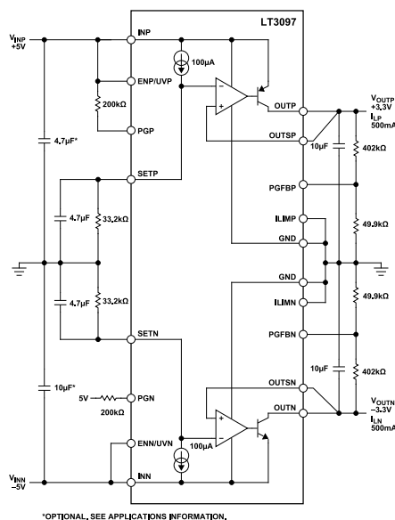
Figure 1. Typical Application
