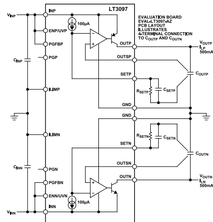
Figure 126. C_{OUTP}/C_{OUTN} and C_{SETP}/C_{SETN} Connections for Best Performance
