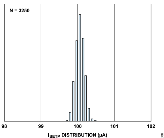
Figure 6. I_{SETP} Distribution
