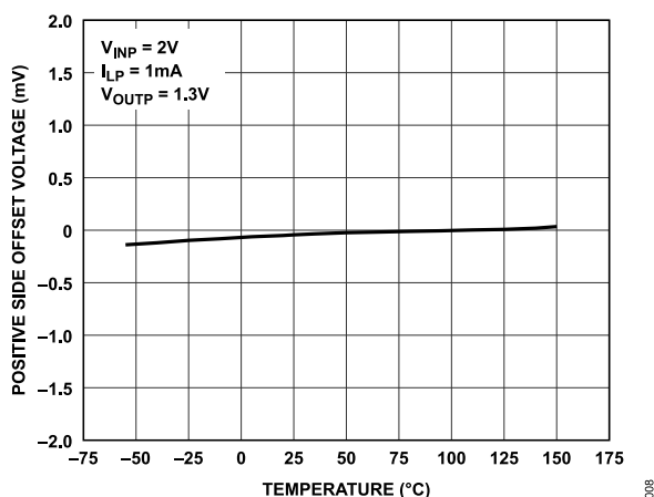
Figure 8. Positive Side Offset Voltage ( V_{OUTP} - V_{SETP} ) vs. Temperature
