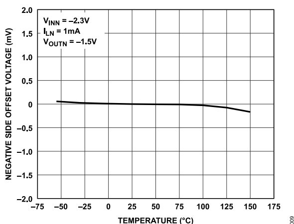
Figure 9. Negative Side Offset Voltage ( V_{OUTN} - V_{SETN} ) vs. Temperature
