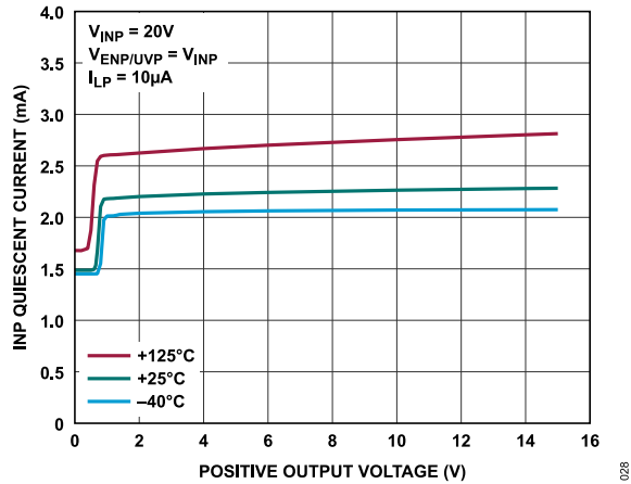
Figure 28. INP Quiescent Current vs. Positive Output Voltage
