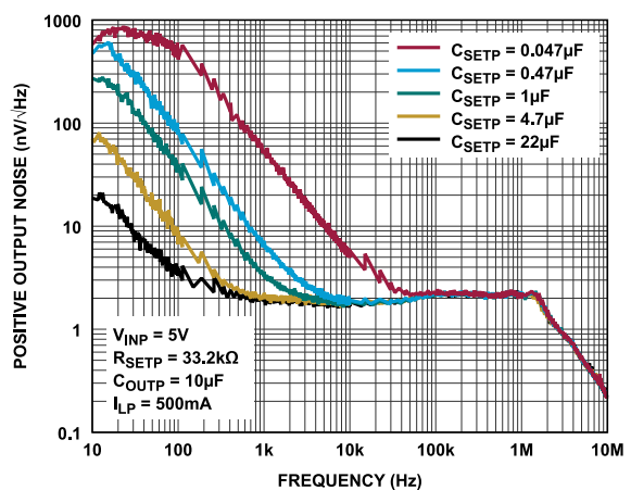
Figure 98. Positive Output Noise vs. Frequency ( C_{SETP} Steps)
