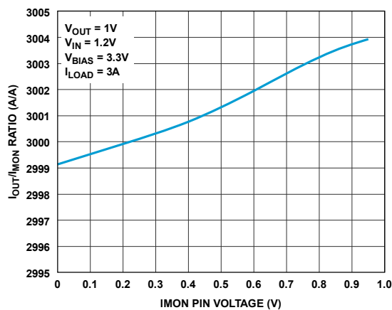
Figure 37. I_{OUT}/I_{MON} Ratio
