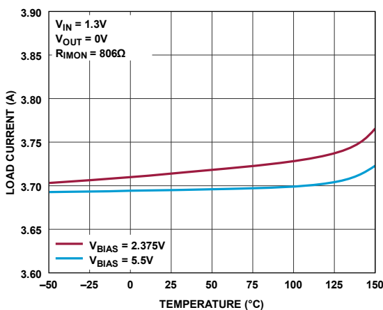
Figure 38. External Current Limit (3.72A)
