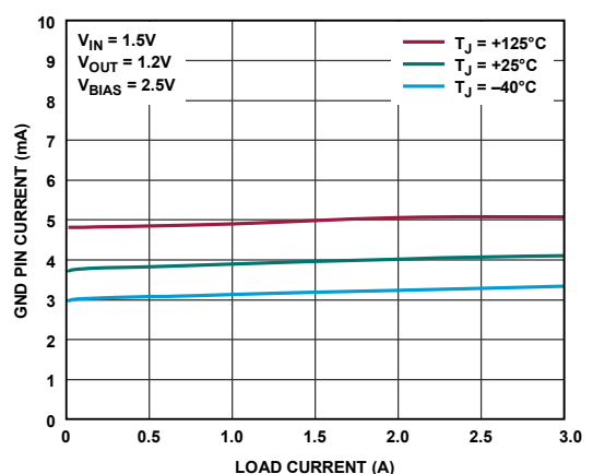
Figure 14. GND Pin Current
