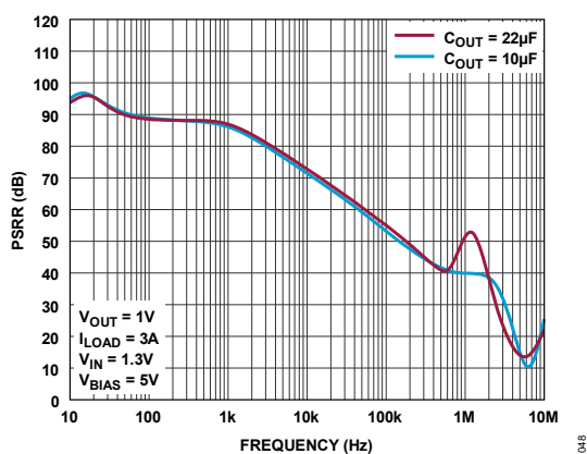
Figure 48. IN Pin PSRR
