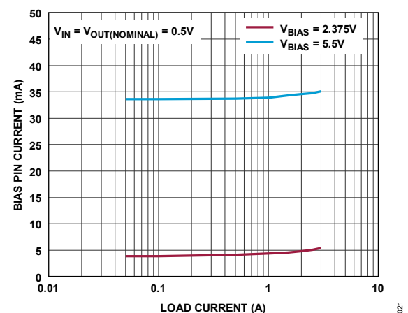
Figure 21. BIAS Pin Current in Dropout
