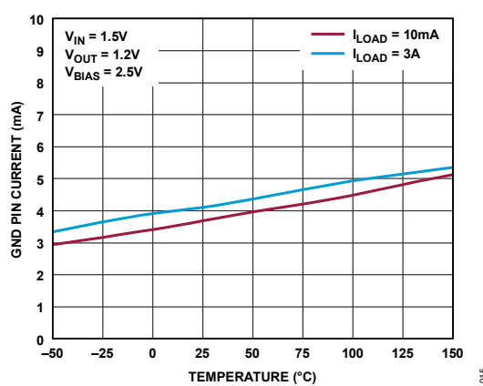
Figure 15. GND Pin Current
