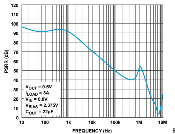
Figure 49. IN Pin PSRR
