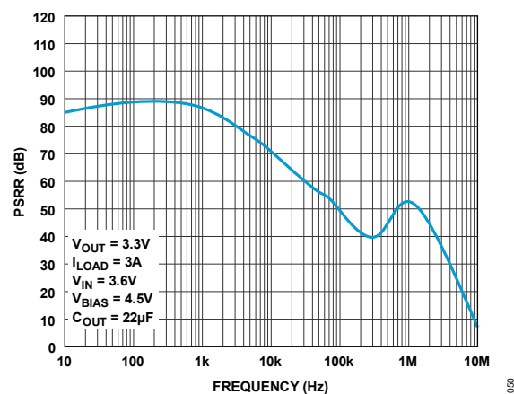
Figure 50. IN Pin PSRR
