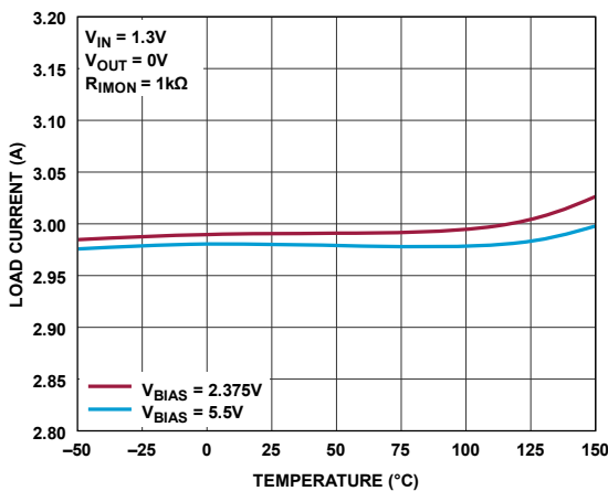
Figure 39. External Current Limit (3A)
