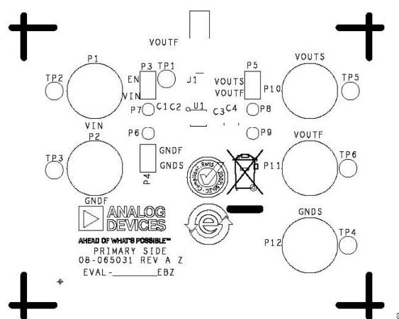
Figure 3. EVAL-ADR3630EBZ Silkscreen
