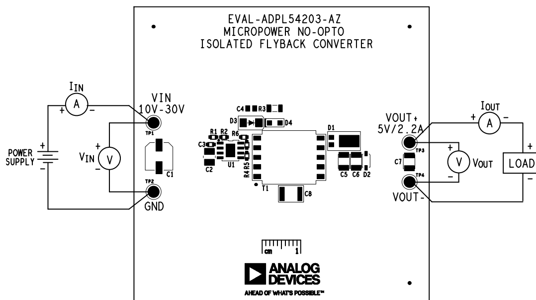
Figure 1. EVAL-ADPL54203-AZ Board Connections
