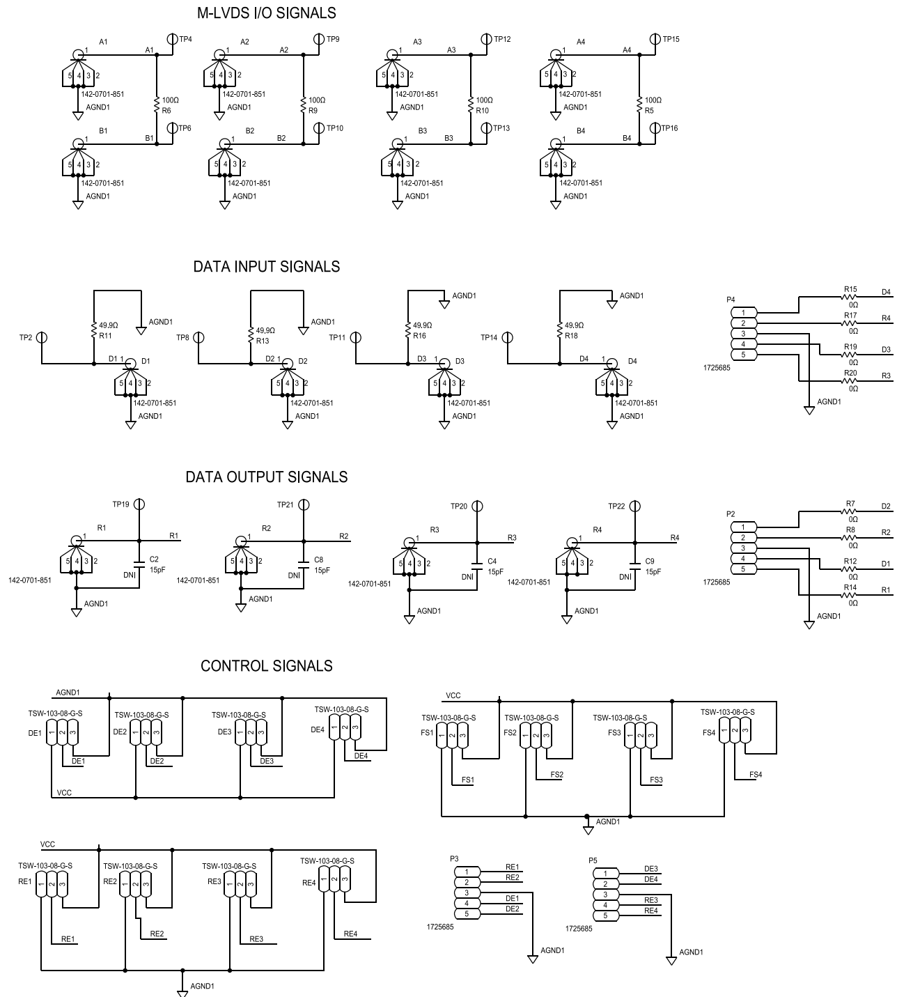
Figure 4. EVAL-ADN4680EEBZ Schematic (Page 2)
