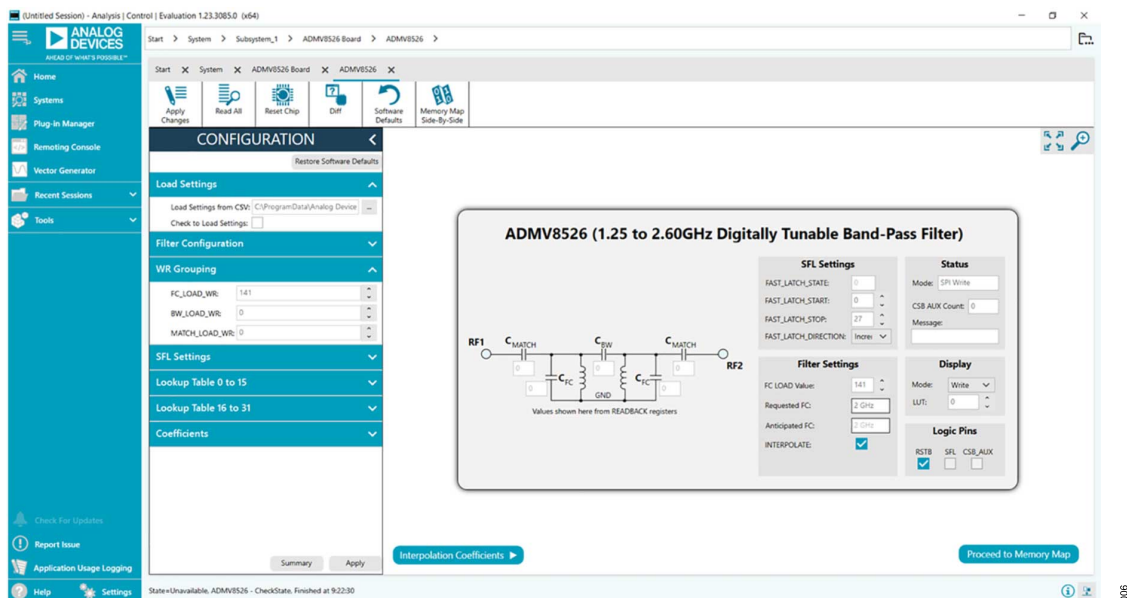
Figure 6. ADMV8526 Chip Plug-In View
