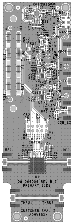
Figure 14. ADMV8526-EVALZ Layer 1
