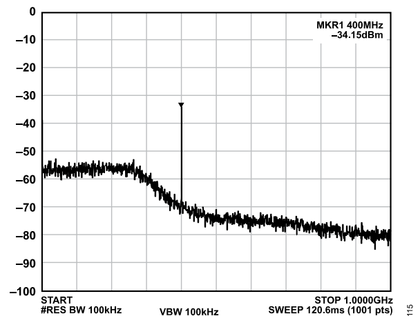
Figure 15. ADMV4540-EVALZ Test Results for f_{RF} = 17.4\text{ GHz} and a 250 MHz SPI-Selectable LPF
