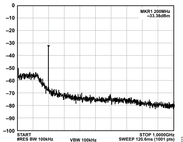
Figure 13. ADMV4540-EVALZ Test Results for f_{RF} = 17.2\text{ GHz} and a 125 MHz SPI-Selectable LPF
