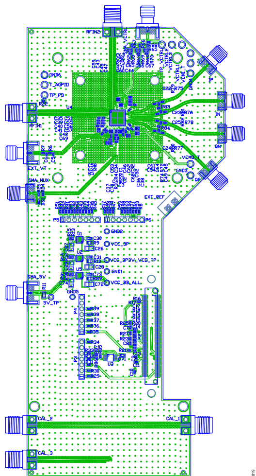
Figure 26. ADMV4540-EVALZ Evaluation Board Top Layer
