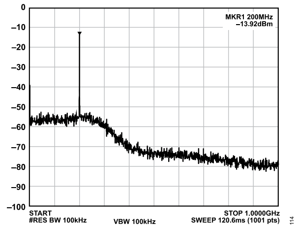
Figure 14. ADMV4540-EVALZ Test Results for f_{RF} = 17.2\text{ GHz} and a 250 MHz SPI-Selectable LPF
