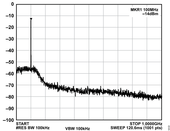
Figure 12. ADMV4540-EVALZ Test Results for f_{RF} = 17.1\text{ GHz} and a 125 MHz SPI-Selectable LPF
