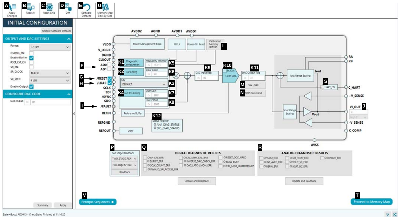
Figure 8. AD5413 Block Diagram with Labels
