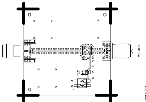
Figure 7. EV-ADF5709 Layer 1
