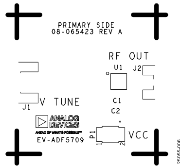
Figure 6. EV-ADF5709 Silkscreen
