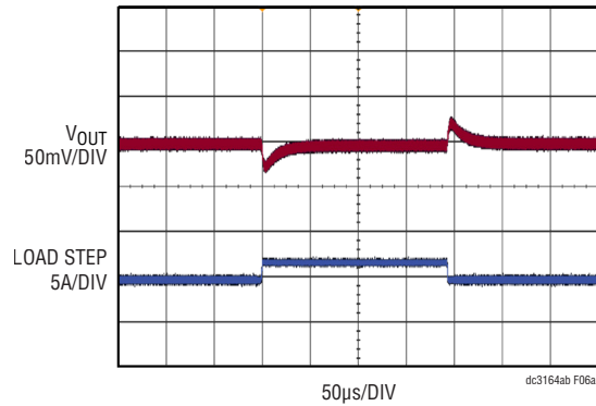
(a) V_{OUT1} = 0.8V
