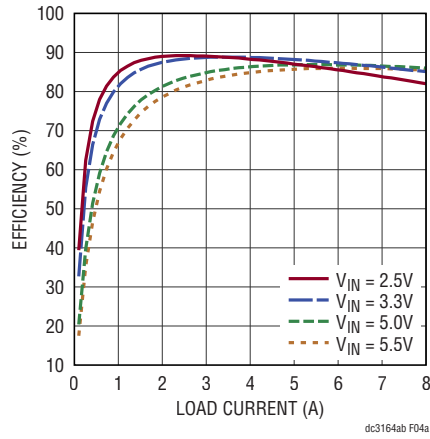
(a) V_{OUT1} = 0.8V
