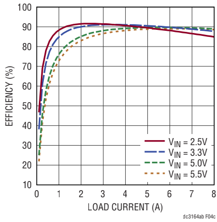
(c) V_{OUT3} = 1.2V
