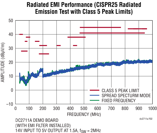
Figure 2. LT8608S Demo Circuit EMI Performance in CISPR25 Radiated Emission Test, Antenna Polarization: Vertical ( V_{IN} = 14\text{V} , V_{OUT} = 5\text{V} , I_{OUT} = 1.5\text{A} , 2MHz Switching Frequency)
