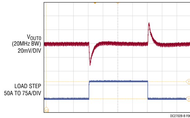
Figure 6. Output Voltage V_{OUT0} vs Load Current ( V_{OUT0} = 1.0V )
