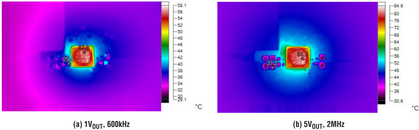
Figure 3. Measured Thermal Capture at 12V_{IN} , I_{OUT} = 12A at 25^{\circ}C Ambient with No Airflow
