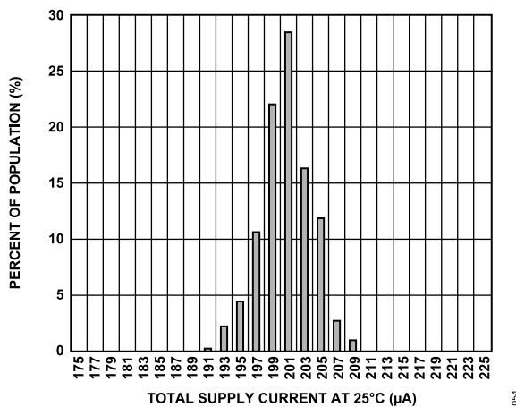
Figure 28. Total Supply Current at 25°C, 3.3 V
