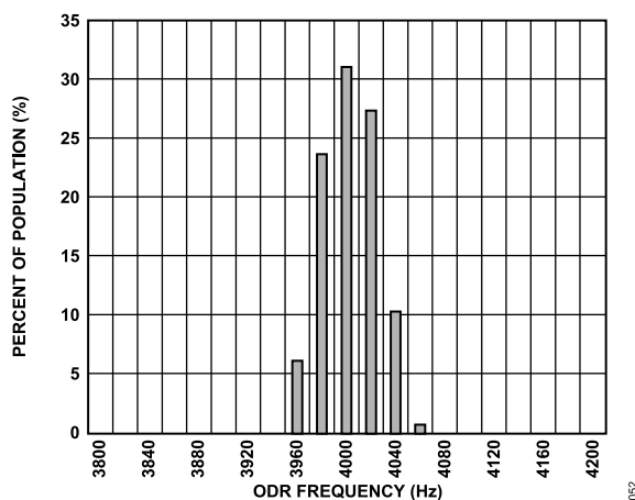
Figure 26. Internal ODR Frequency Histogram
