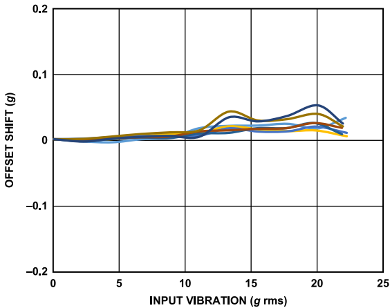
Figure 22. VRE, Y-Axis Offset from -1 g, \pm 40 g Range, Y-Axis Orientation = -1 g
