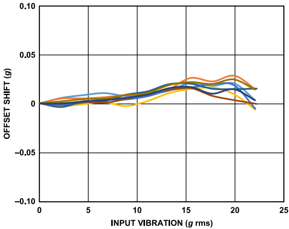
Figure 21. VRE, X-Axis Offset from -1 g, \pm 40 g Range, X-Axis Orientation = -1 g
