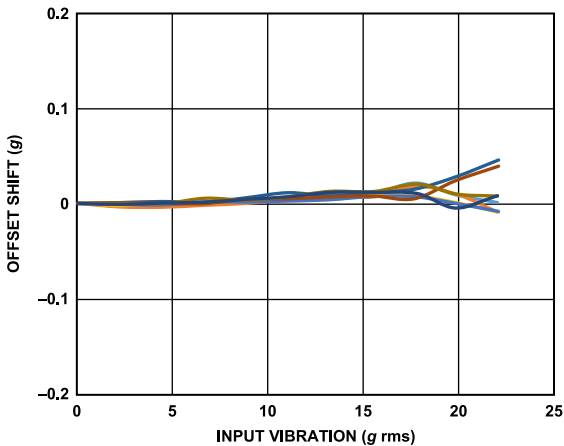
Figure 23. VRE, Z-Axis Offset from -1 g, \pm 40 g Range, Z-Axis Orientation = -1 g
