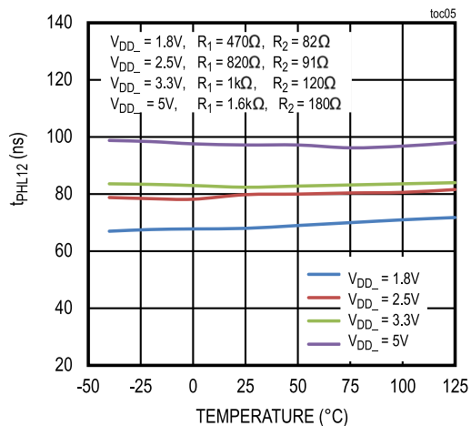
PROPAGATION DELAY t_{PHL12} vs. TEMPERATURE
