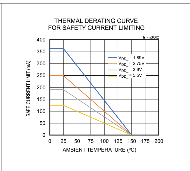
Figure 4. Thermal Derating Curve for Safety Current Limiting for 8-Lead Narrow SOIC Package
