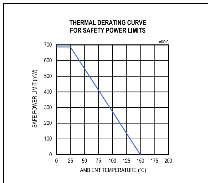
Figure 3. Thermal Derating Curve for 8-Lead Narrow SOIC Package
