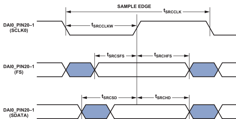
Figure 20. ASRC Serial Input Port Timing
