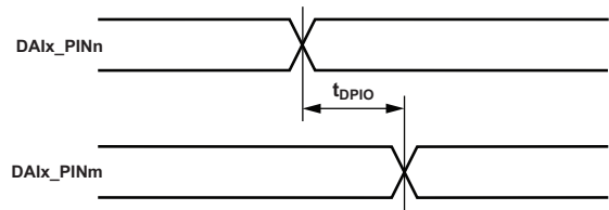
Figure 33. DAI Pin to DAI Pin Direct Routing
