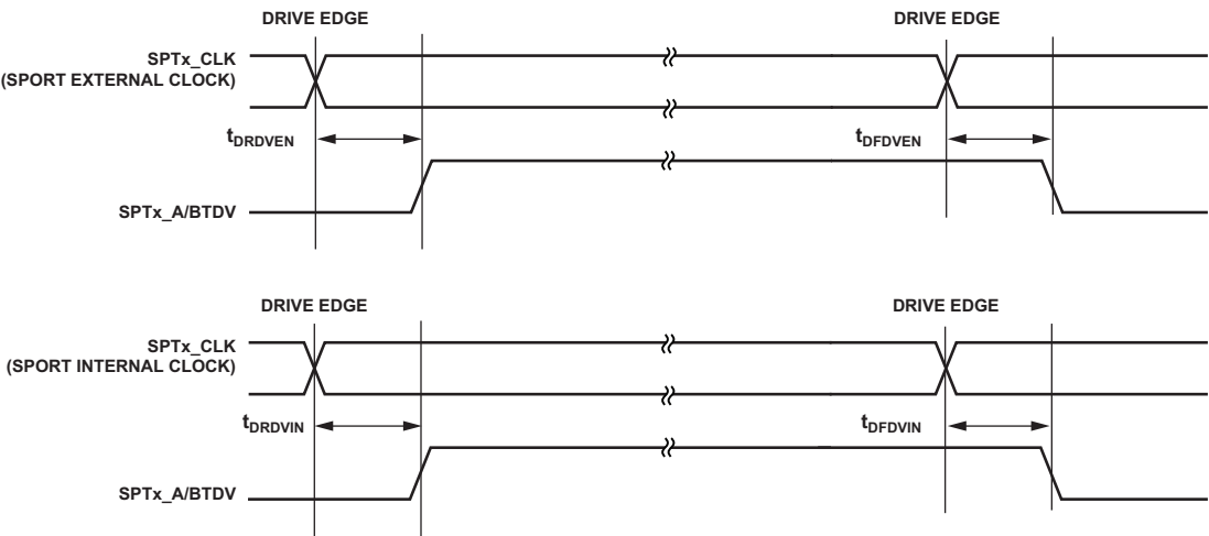
Figure 18. SPORTs—Transmit Data Valid Internal and External Clock
