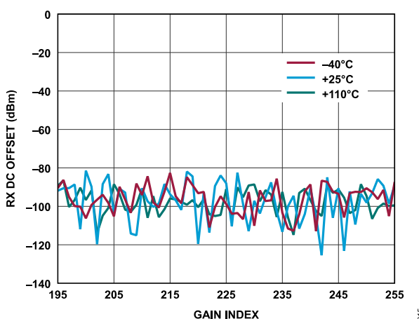
Figure 124. Receiver DC Offset vs. Gain Index, Baseband Frequency = 5.6 MHz, ADC = High Performance
