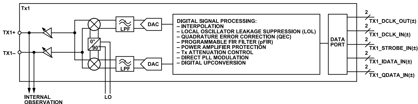
Figure 360. Transmitter Architecture
