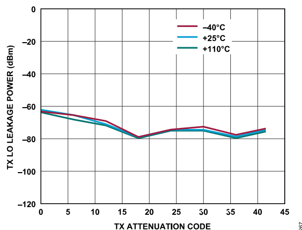
Figure 175. Transmitter LO Leakage Power vs. Transmitter Attenuation Code, Baseband Frequency = 18 MHz, Backoff = 6 dBFS, Initialization Calibration Only
