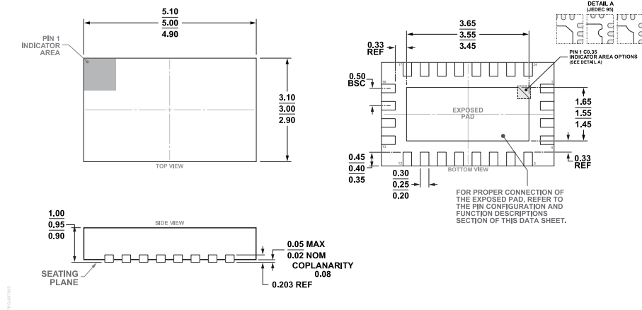
Figure 21. 24-Lead Lead Frame Chip Scale Package [LFCSP] 5 mm x 3 mm Body and 0.95 mm Package Height (CP-24-27) Dimensions shown in millimeters
