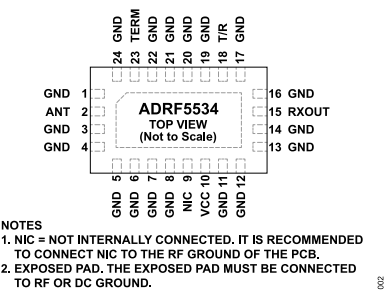
Figure 2. Pin Configuration
