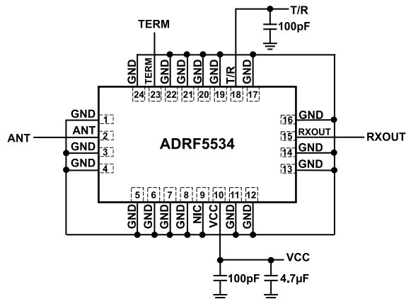
Figure 17. Recommended Schematic
