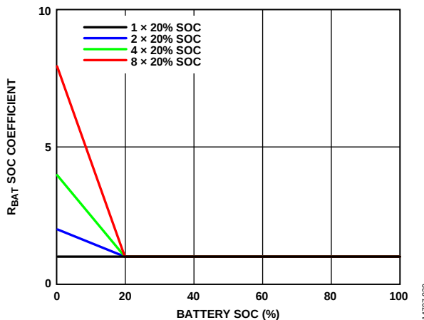
Figure 46. R_{\text{BAT}} SOC Coefficient vs. Battery SOC, SOC Coefficient of the Li-Ion Battery, Relative to Battery R_{\text{BAT}} at 25°C
