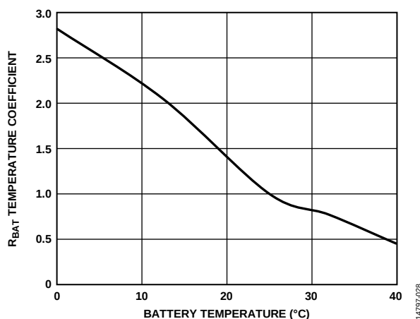
Figure 45. R_{\text{BAT}} Temperature Coefficient vs. Battery Temperature, Temperature Coefficient of the Li-Ion Battery, Relative to Battery R_{\text{BAT}} at 25°C
