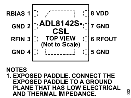
Figure 2. Pin Configuration
