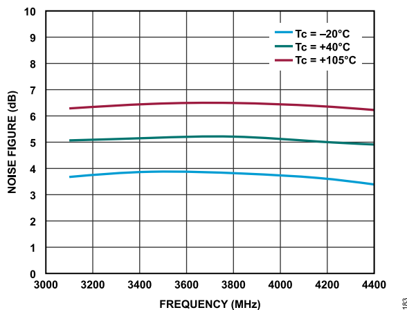
Figure 83. Noise Figure vs. Frequency for Various Temperatures
