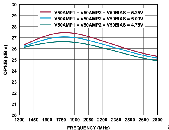
Figure 43. OP1dB vs. Frequency for Various Supplies
