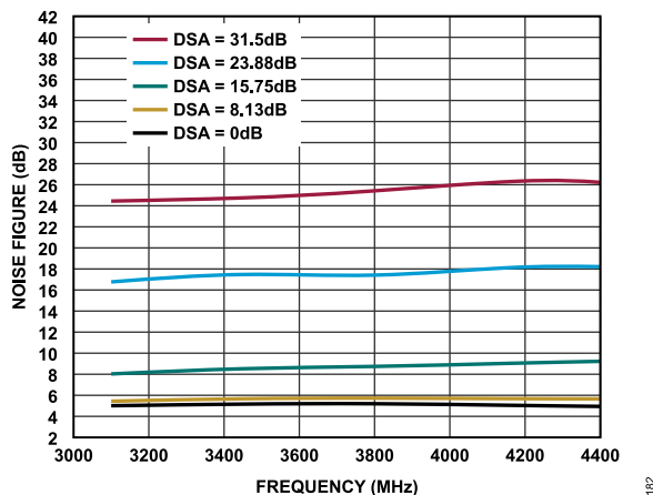
Figure 82. Noise Figure vs. Frequency at Various DSA Values
