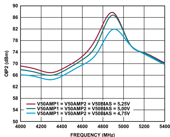
Figure 104. OIP2 vs. Frequency for Various Supplies
