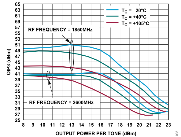
Figure 49. OIP3 vs. Output Power Per Tone for Various Temperatures at 1850 MHz and 2600 MHz
