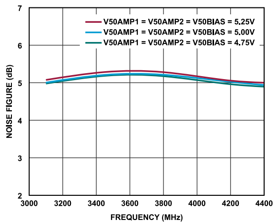
Figure 81. Noise Figure vs. Frequency for Various Supplies
