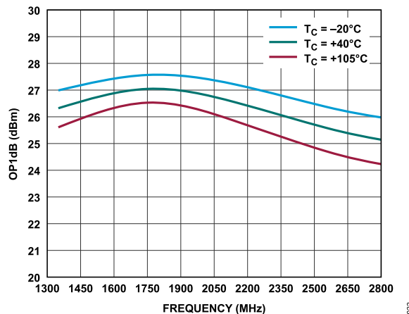
Figure 44. OP1dB vs. Frequency for Various Temperatures
