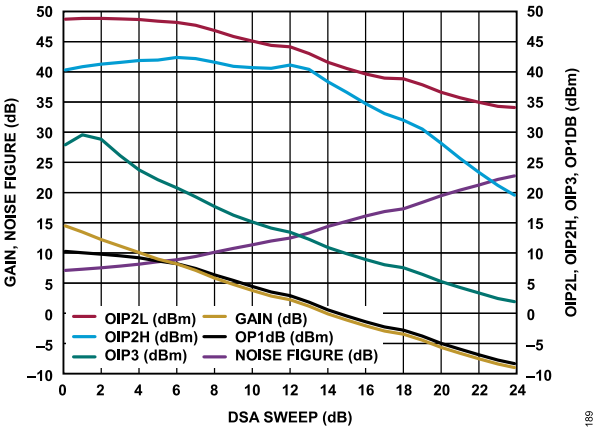
Figure 89. Gain, Noise Figure, OIP2L, OIP2H, OIP3, OP1dB vs. DSA Sweep, Frequency = 12000 MHz
