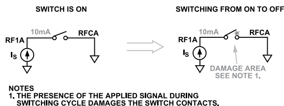
Figure 65. Hot Switching Condition When Turning the Switch from On to Off
