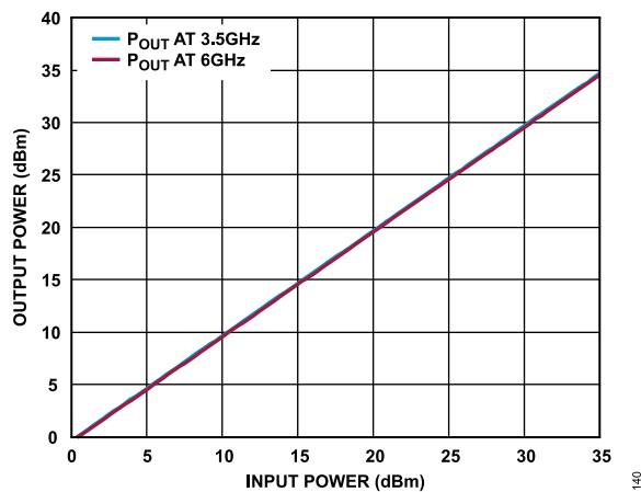
Figure 43. Output Power ( P_{OUT} ) vs. Input Power ( P_{IN} ) ( V_{DD} = 3.3 V)
