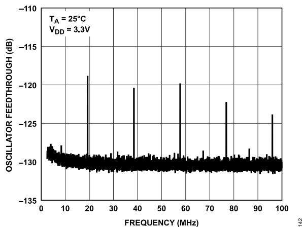
Figure 45. Oscillator Feedthrough vs. Frequency, Wide Bandwidth ( V_{DD} = 3.3 V)
