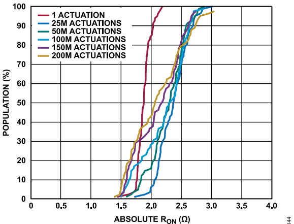
Figure 63. Population vs. Absolute R_{ON} , Switch Actuated at 85°C and R_{ON} Measured at 25°C, Actuation Frequency = 289 Hz, V_{DD} = 3.3 V
