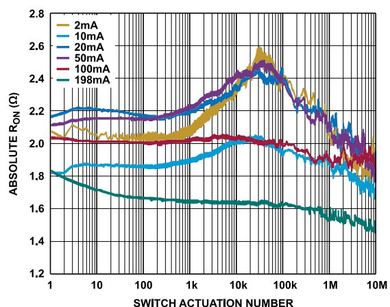
Figure 9. Absolute R_{ON} vs. Switch Actuation Number Over Different Currents Applied During Actuations ( T_A = 25^\circ\text{C} , V_{DD} = 3.3\text{ V} )
