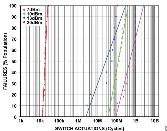
Figure 67. RF Hot Switching Probability Distribution on Log Normal (RF Power = Continuous Wave, Terminated into 50 Ω, T_A = 25^\circ\text{C} , V_{DD} = 3.3\text{ V} )
