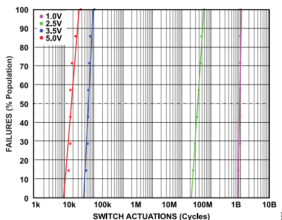
Figure 69. DC Hot Switching Probability Distribution on Log Normal (Terminated into 50 Ω, T_A = 25^\circ\text{C} , V_{DD} = 3.3\text{ V} )
