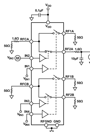
Figure 68. DC Hot Switching Setup
