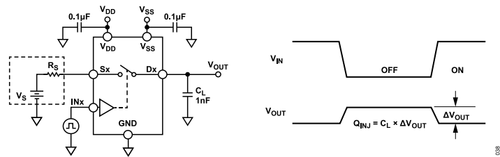
Figure 38. Charge Injection
