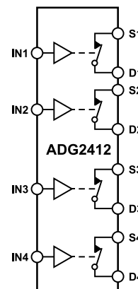
Figure 1. Functional Block Diagram
