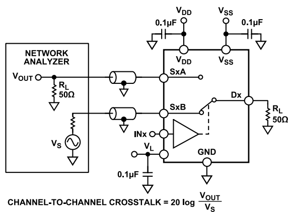
Figure 31. Channel-to-Channel Crosstalk
