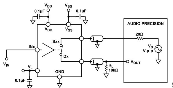
Figure 32. THD + Noise
