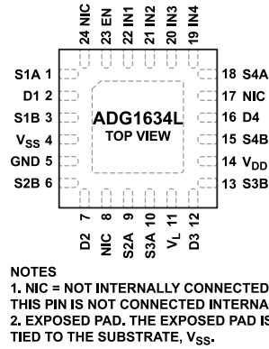
Figure 2. Pin Configuration
