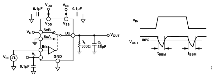
Figure 26. Break-Before-Make Delay, t_{BBM}
