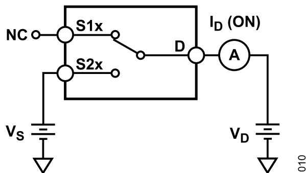
Figure 24. On Leakage
