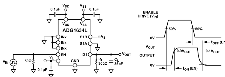
Figure 27. Enable Delay On Time, t_{ON} (EN) and Enable Delay Off Time, t_{OFF} (EN)
