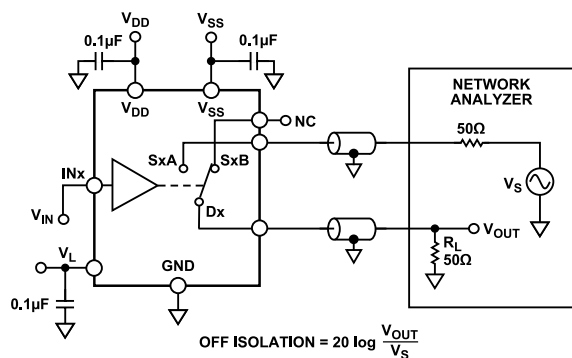
Figure 29. Off Isolation
