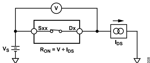
Figure 22. On Resistance
