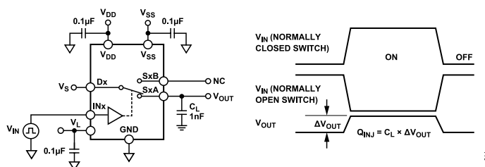
Figure 28. Charge Injection
