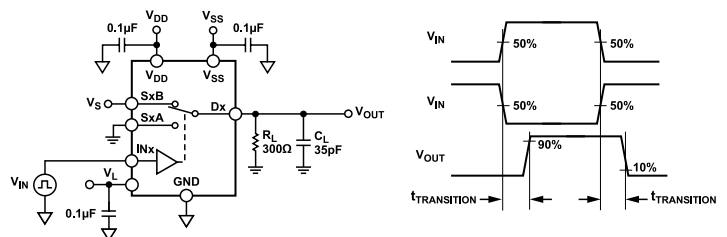
Figure 25. Transition Time, t_{TRANSITION} ( V_{IN} Is the Input Voltage, and V_{OUT} Is the Output Voltage.)
