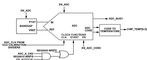
Figure 76. Temperature Sensor
