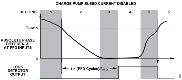
Figure 67. Lock Detector Timing, Bleed Current Disabled
