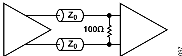
Figure 97. Far-End Transmission Line Termination ( Z_0 = 50 \Omega )
