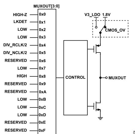
Figure 75. MUXOUT
