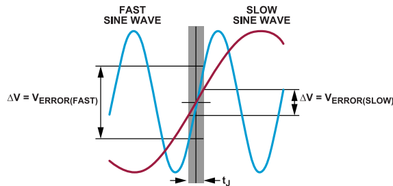
Figure 94. Fast and Slow Sine Wave Signals Sampled with a Jittery Clock
