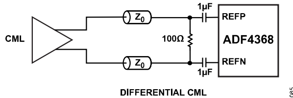
Figure 48. Differential CML
