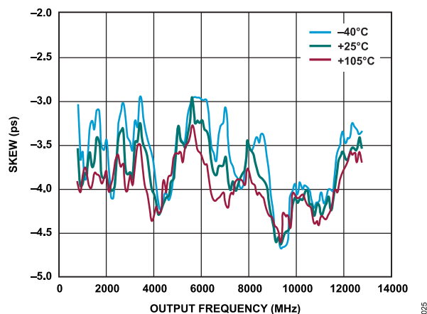
Figure 25. Skew Between Outputs
