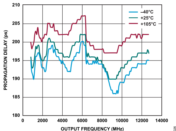
Figure 26. Propagation Delay
