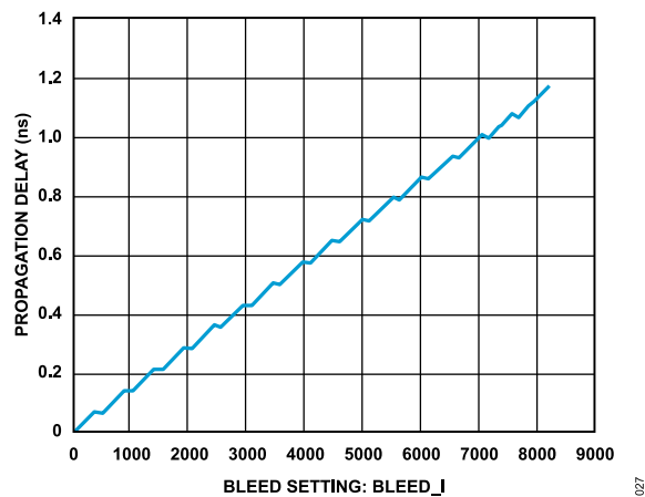
Figure 27. Propagation Delay vs. Bleed Setting
