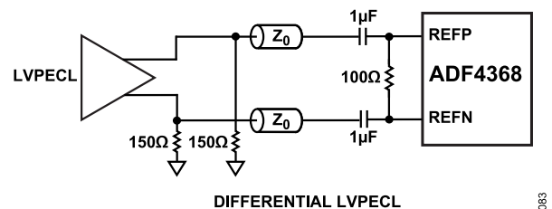
Figure 46. Differential LVPECL
