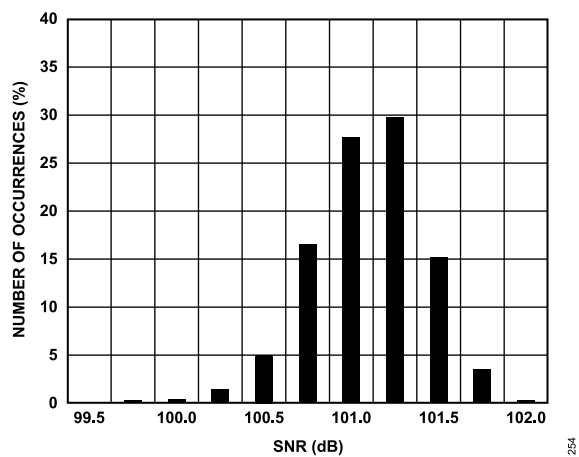
Figure 36. SNR Histogram of ADC SNR for 1000 Devices Tested at T_A = 25^\circ\text{C} with PGA_GAIN = 1 and 8 kSPS Data Rate
