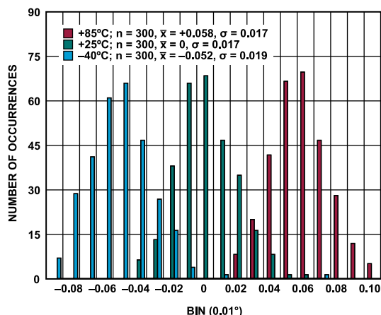
Figure 70. Device-to-Device Phase Angle Mismatch, 20 kHz, AFE_GAIN = 2.6 V/V (Gain 3 Mode), Normalized to the Mean Value at 25°C
