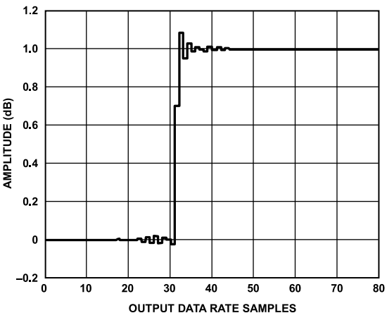
Figure 122. Wideband Low Ripple FIR Filter Step Response
