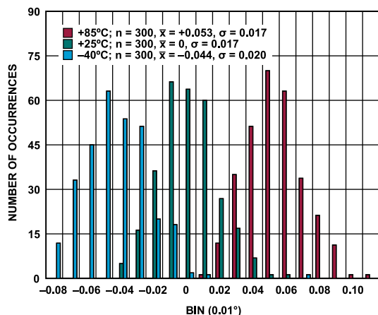
Figure 68. Device-to-Device Phase Angle Mismatch, 20 kHz, AFE_GAIN = 0.65 V/V (Gain 1 Mode), Normalized to the Mean Value at 25°C
