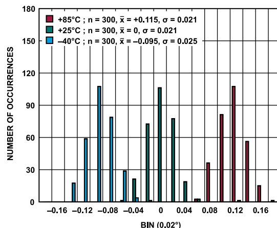
Figure 73. Device-to-Device Phase Angle Mismatch, 20 kHz, AFE_GAIN = 20.8 V/V (Gain 6 Mode), Normalized to the Mean Value at 25°C
