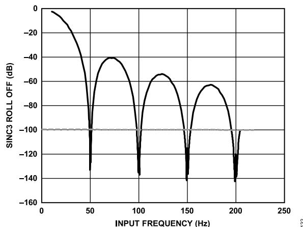
Figure 128. Sinc3 Filter Frequency Response Showing 50 Hz Rejection, 50 Hz ODR, x163,840 Decimation
