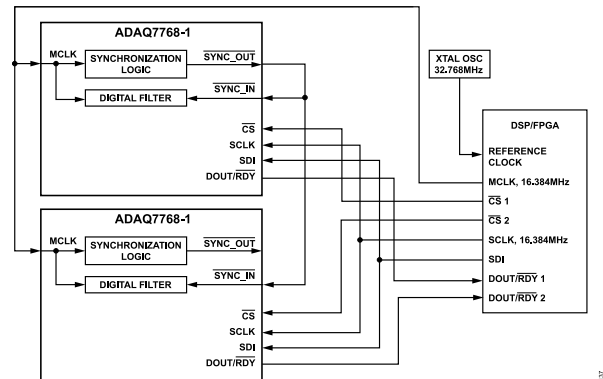
Figure 133. Basic SPI Synchronization Diagram
