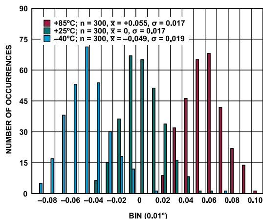
Figure 69. Device-to-Device Phase Angle Mismatch, 20 kHz, AFE_GAIN = 1.3 V/V (Gain 2 Mode), Normalized to the Mean Value at 25°C
