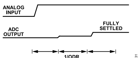
Figure 127. Sinc3 Filter Step Response
