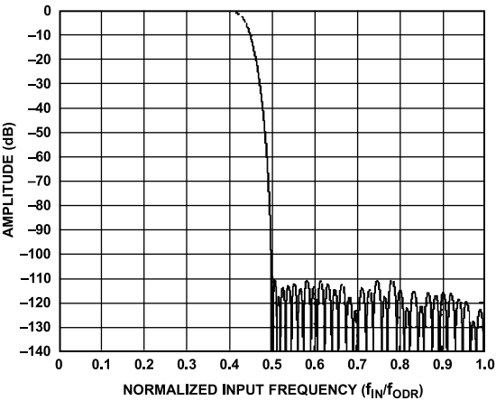
Figure 120. Low Ripple FIR Filter Frequency Response
