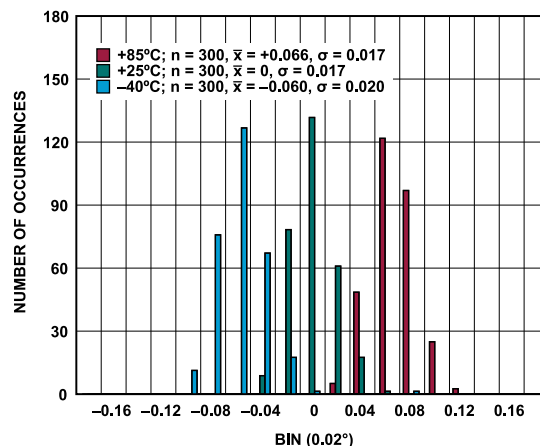
Figure 71. Device-to-Device Phase Angle Mismatch, 20 kHz, AFE_GAIN = 5.2 V/V (Gain 4 Mode), Normalized to the Mean Value at 25°C
