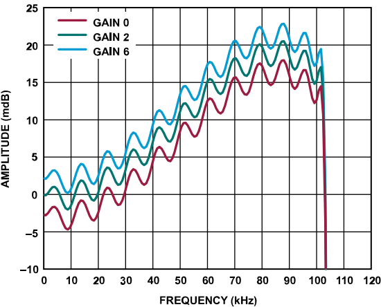
Figure 121. Wideband Low Ripple FIR Filter Passband Ripple, Normalized to Gain 2 Mode
