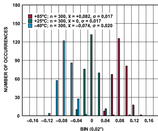
Figure 72. Device-to-Device Phase Angle Mismatch, 20 kHz, AFE_GAIN = 10.4 V/V (Gain 5 Mode), Normalized to the Mean Value at 25°C
