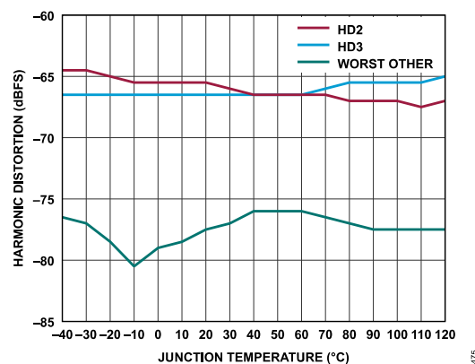
Figure 72. Harmonic Distortion vs. Junction Temperature, f_{IN} = 1.8 GHz, A_{IN} = -1 dBFS, Full Bandwidth Mode
