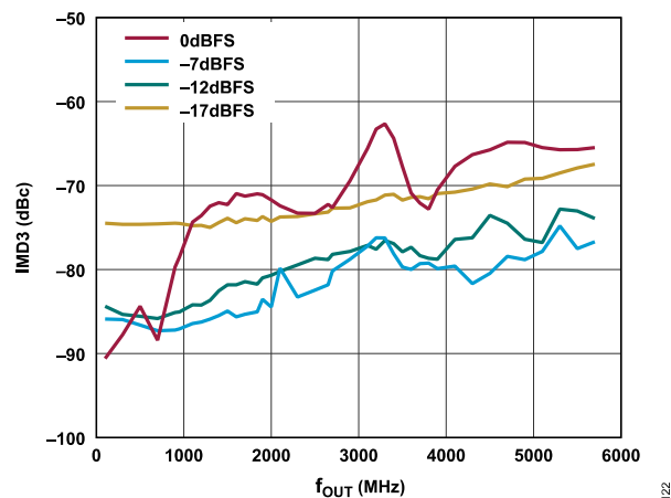
Figure 22. IMD3 vs. f_{OUT} over Digital Scale, 12 GSPS DAC Sample Rate, Channel Interpolation 4x, Main Interpolation 8x, 16B Mode, IMD3 is a Two-Tone Test, and the Scale per Tone is 6 dB Lower than the Reported Digital Scale
