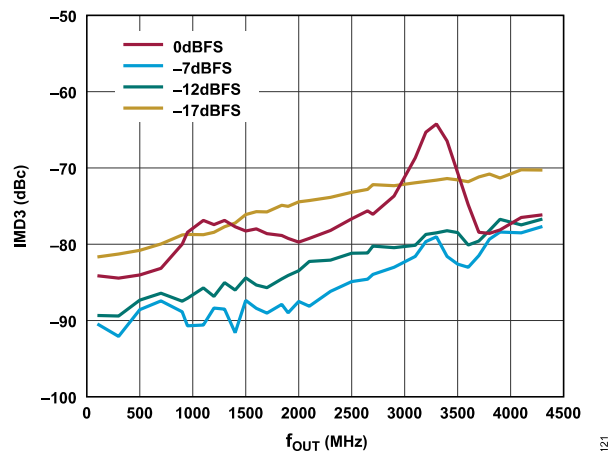
Figure 21. IMD3 vs. f_{OUT} over Digital Scale, 9 GSPS DAC Sample Rate, Channel Interpolation 1x, Main Interpolation 6x, 15C Mode, IMD3 is a Two-Tone Test, and the Scale per Tone is 6 dB Lower than the Reported Digital Scale
