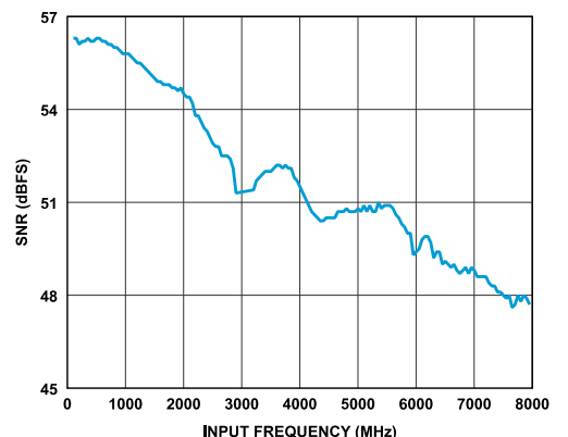
Figure 64. SNR vs. Input Frequency with A_{IN} = -1 dBFS, Full Bandwidth Mode
