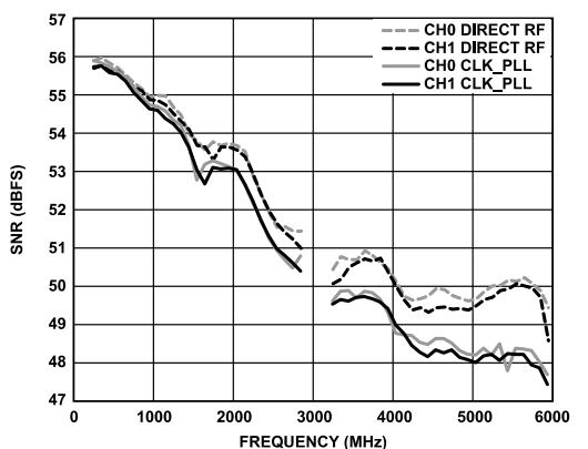
Figure 59. SNR vs. Frequency with A_{IN} = -1 dBFS, Full Bandwidth Mode
