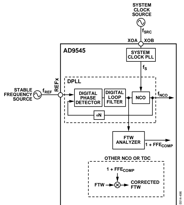
Figure 103. Closed-Loop Method
