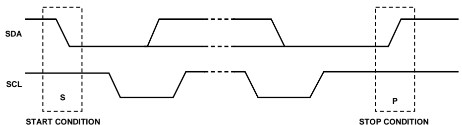
Figure 129. Start and Stop Conditions
