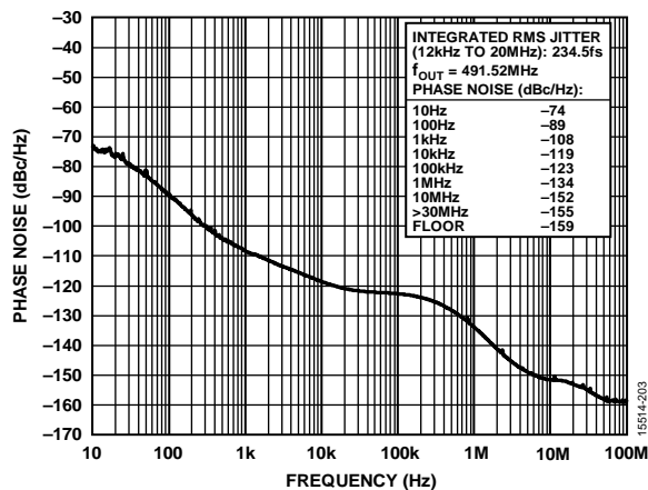
Figure 5. Absolute Phase Noise (PLL0, Configuration 3, HCSSL Mode, f_{REF} = 1\text{ Hz} , f_{OUT} = 491.52\text{ MHz} , f_{COMP} = 19.2\text{ MHz} TCXO, f_{OSC} = 52\text{ MHz} Crystal, 0.05 Hz DPLL BW)
