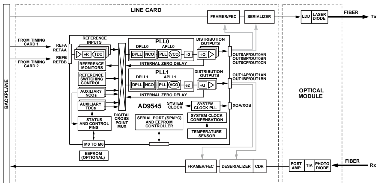
Figure 115. Optical Line Card Direct Timing Example
