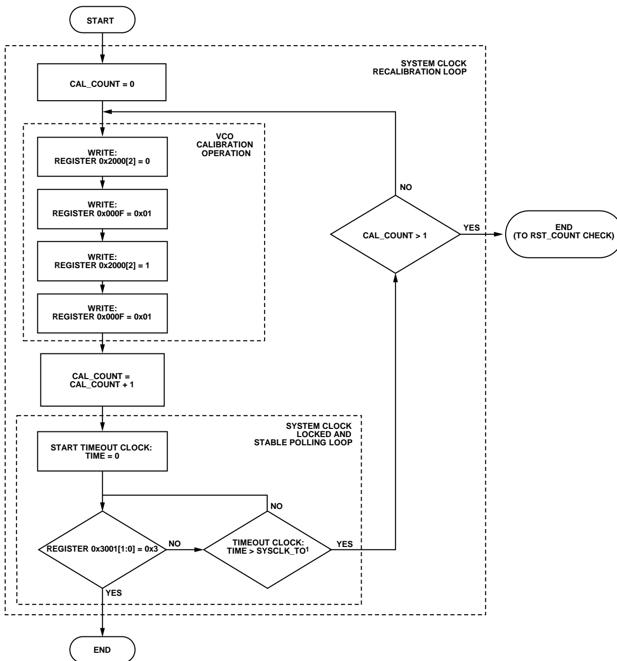
Figure 120. AD9545 System Clock Initialization Subprocess
