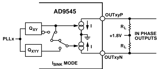
Figure 44. Single-Divider, Single-Ended Mode Providing In-Phase Outputs (Current Sink Mode)
