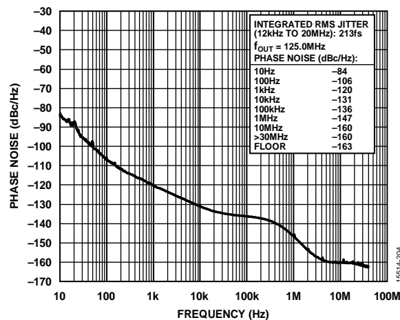
Figure 6. Absolute Phase Noise (PLL0, Configuration 4, HCSSL Mode, f_{REF} = 125\text{ MHz} , f_{OUT} = 125.0\text{ MHz} , f_{COMP} = 19.2\text{ MHz} TCXO, f_{OSC} = 52\text{ MHz} Crystal, 0.1 Hz DPLL BW, Phase Buildout Mode)
