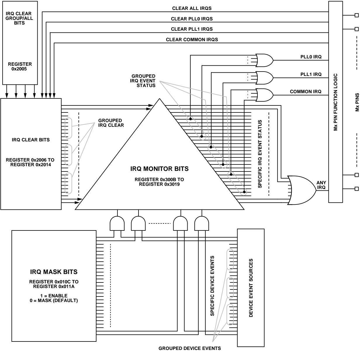
Figure 111. IRQ System Diagram
