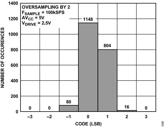
Figure 50. Histogram of Codes—OS x 2 (Four Codes)
