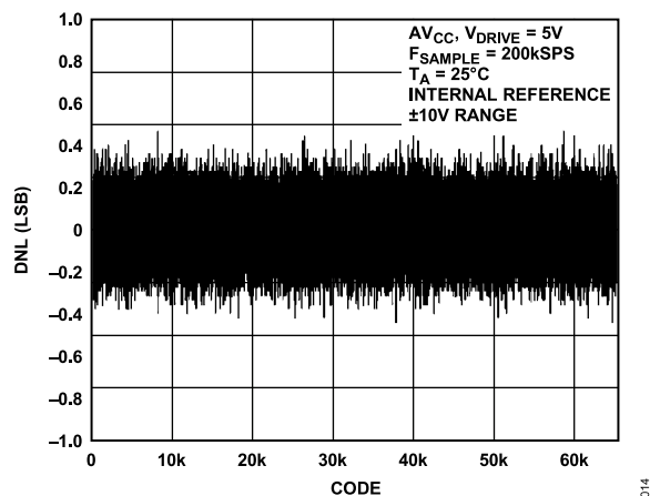
Figure 15. AD7606 Typical DNL, \pm 10 V Range
