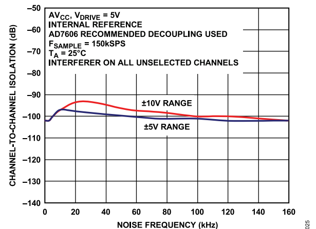
Figure 28. Channel-to-Channel Isolation
