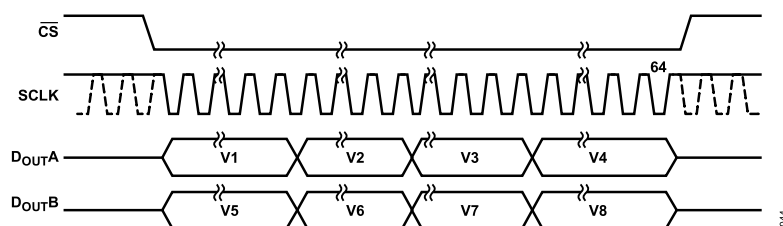
Figure 46. AD7606 Serial Interface with Two D_{OUT} Lines
