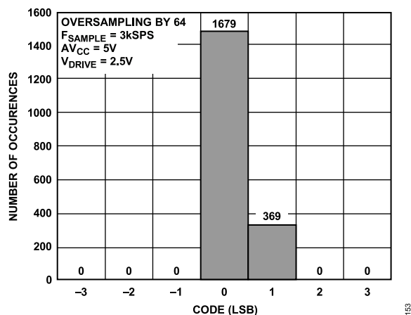
Figure 55. Histogram of Codes—OS × 64 (Two Codes)
