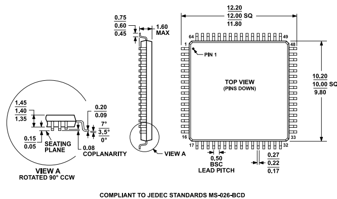
Figure 65. 64-Lead Low Profile Quad Flat Package [LQFP] (ST-64-2) Dimensions shown in millimeters
