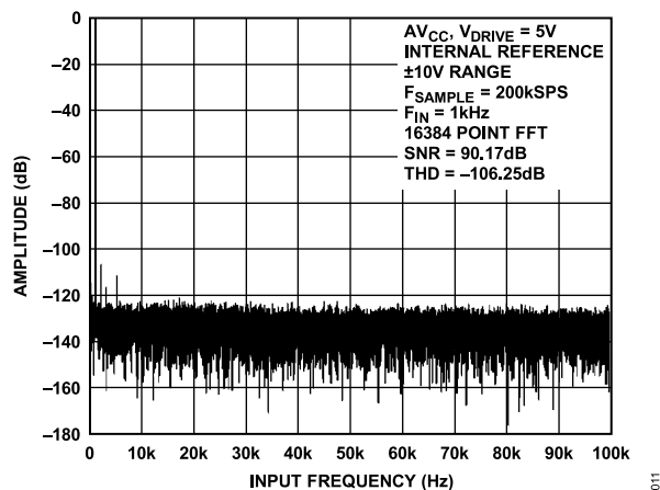
Figure 11. AD7606 FFT, \pm 10 V Range
