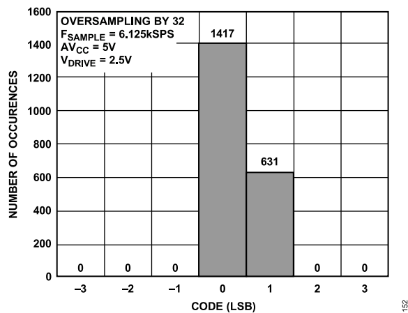
Figure 54. Histogram of Codes—OS × 32 (Two Codes)
