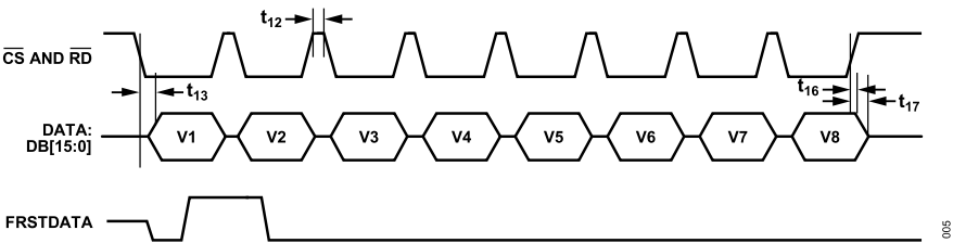
Figure 5. CS and RD, Linked Parallel Mode
