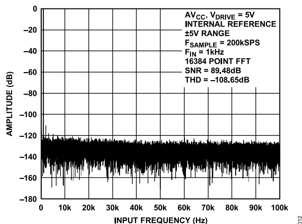
Figure 12. AD7606 FFT Plot, \pm 5 V Range
