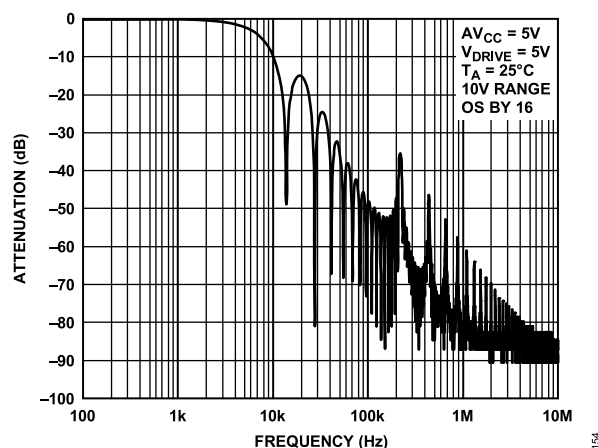
Figure 59. Digital Filter Response for OS 16
