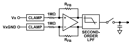
Figure 34. Analog Input Circuitry
