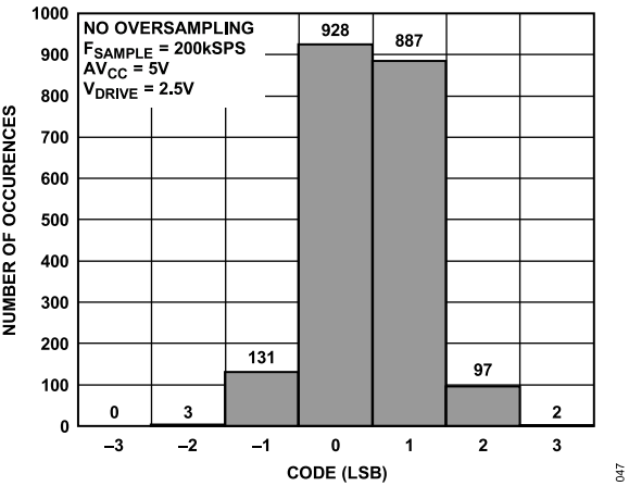
Figure 49. Histogram of Codes—No OS (Six Codes)
