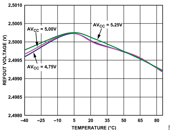
Figure 30. Reference Output Voltage vs. Temperature for Different Supply Voltages
