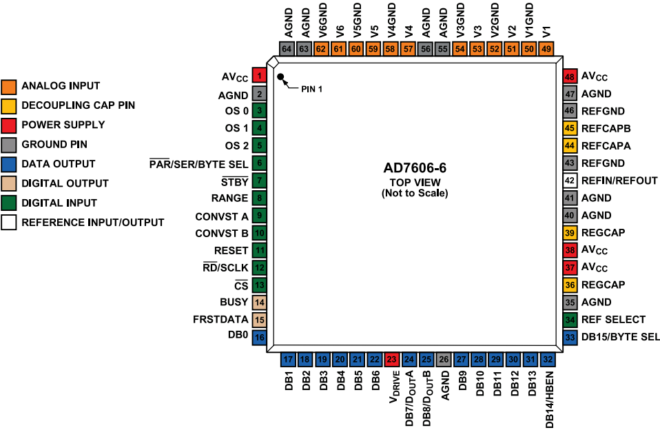
Figure 9. AD7606-6 Pin Configuration
