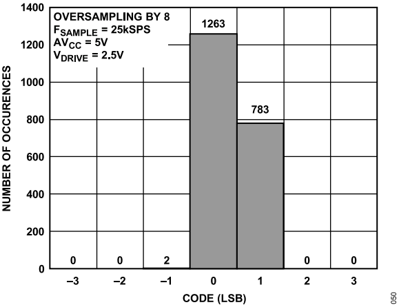
Figure 52. Histogram of Codes—OS x 8 (Three Codes)
