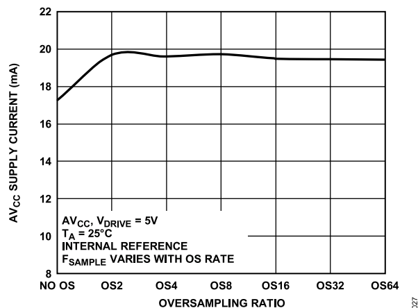
Figure 32. Supply Current vs. Oversampling Rate
