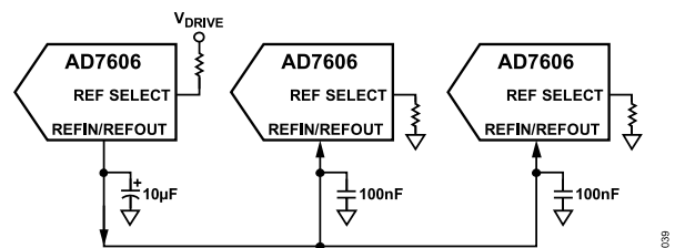
Figure 42. Internal Reference Driving Multiple AD7606/AD7606-6/AD7606-4 REFIN Pins
