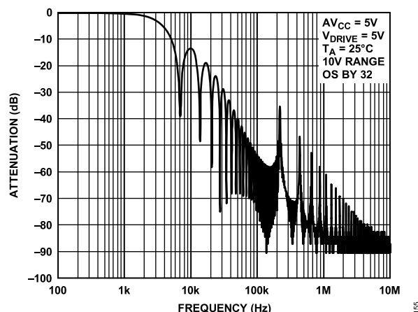
Figure 60. Digital Filter Response for OS 32
