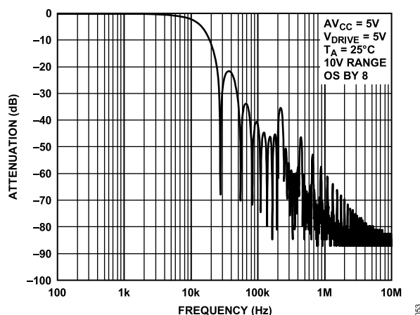
Figure 58. Digital Filter Response for OS 8
