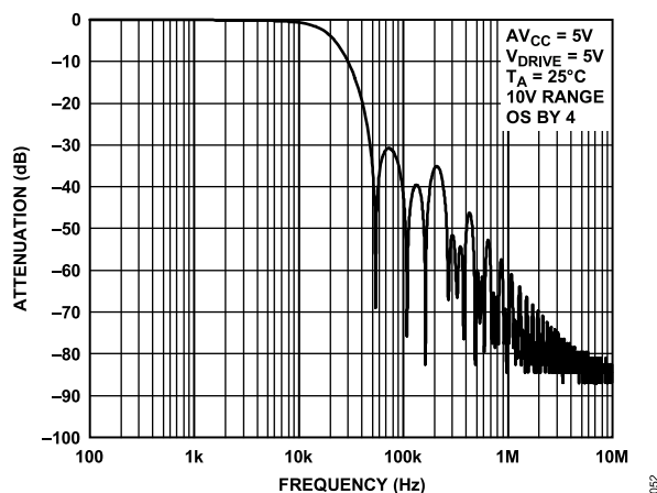
Figure 57. Digital Filter Response for OS 4
