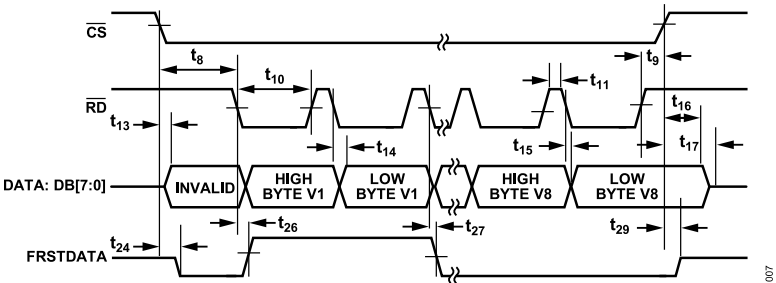
Figure 7. BYTE Mode Read Operation
