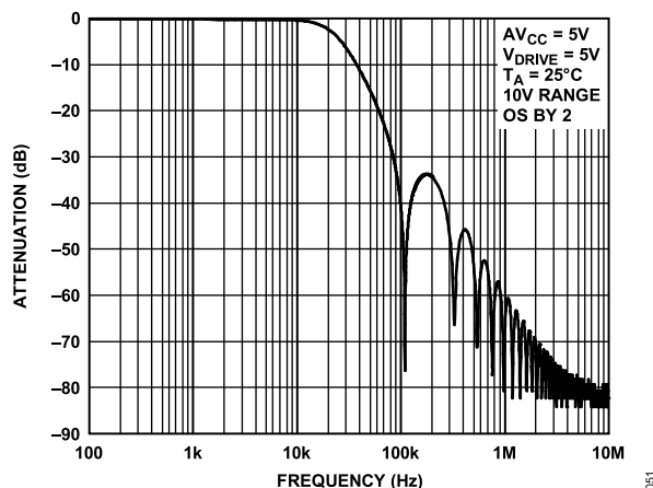
Figure 56. Digital Filter Response for OS 2
