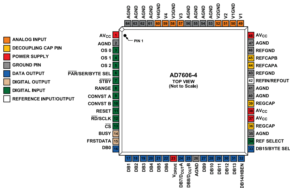
Figure 10. AD7606-4 Pin Configuration
