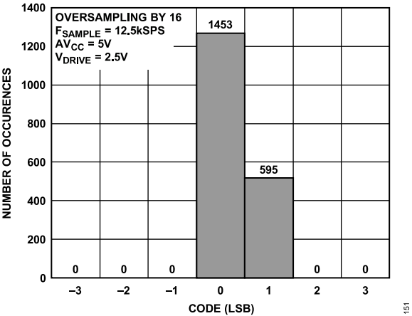
Figure 53. Histogram of Codes—OS x 16 (Two Codes)
