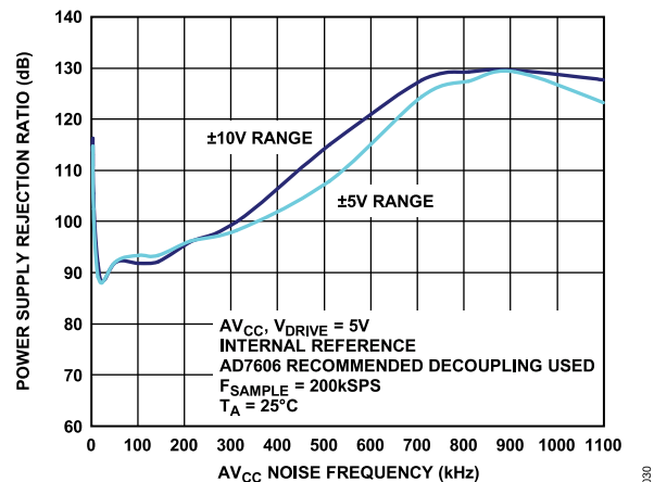
Figure 33. PSRR
