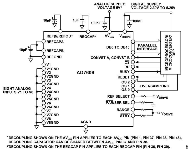
Figure 43. AD7606 Typical Connection Diagram
