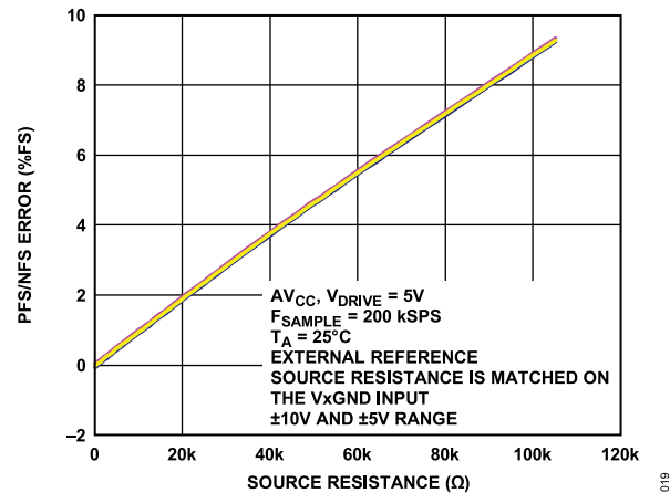
Figure 21. PFS and NFS Error vs. Source Resistance
