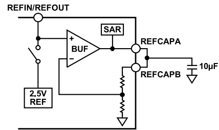
Figure 40. Reference Circuitry
