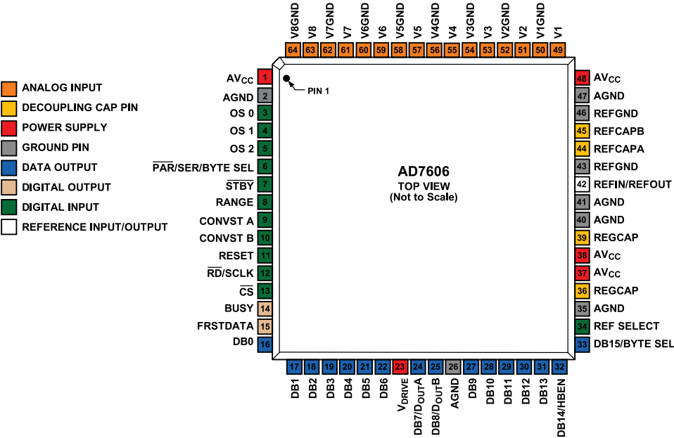
Figure 8. AD7606 Pin Configuration
