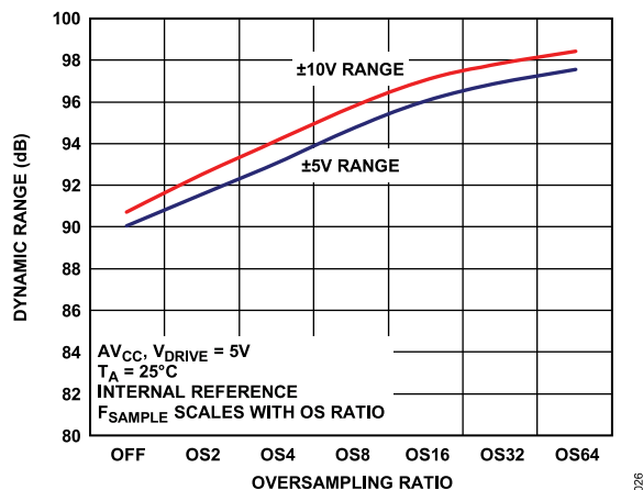
Figure 29. Dynamic Range vs. Oversampling Rate
