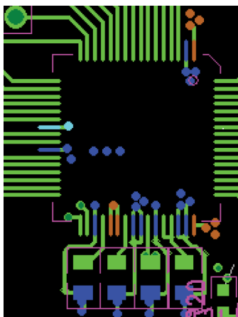
Figure 62. Top Layer Decoupling REFOUT/REFOUT, REFCAP, REFCAPB, and REGCAP Pins
