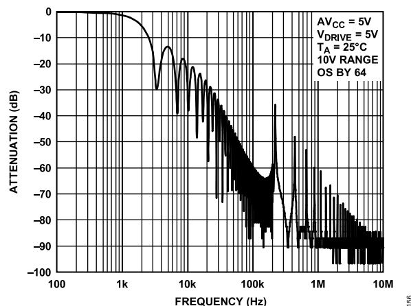
Figure 61. Digital Filter Response for OS 64
