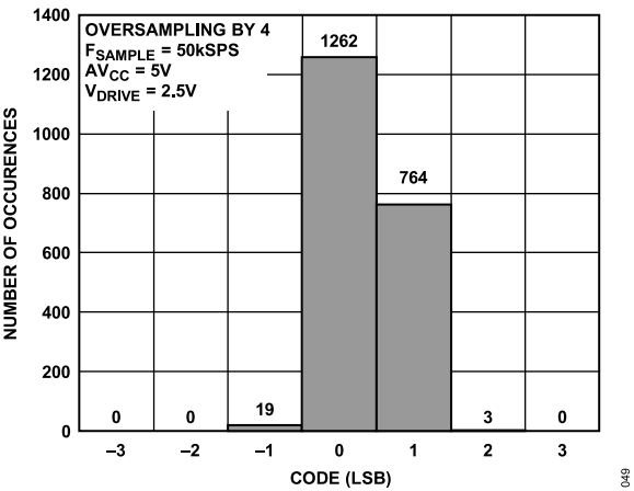
Figure 51. Histogram of Codes—OS x 4 (Four Codes)
