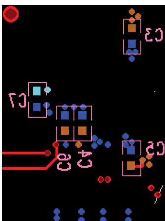
Figure 63. Bottom Layer Decoupling
