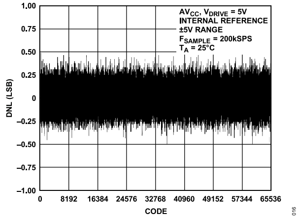
Figure 17. AD7606 Typical DNL, \pm 5 V Range
