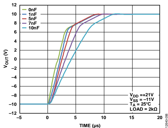
Figure 45. Settling Time vs. Capacitive Load, \pm 10 V Range
