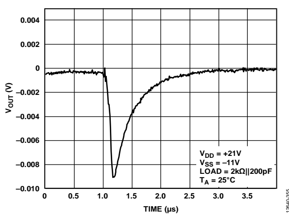
Figure 48. Digital-to-Analog Glitch Energy, \pm 10 V Range
