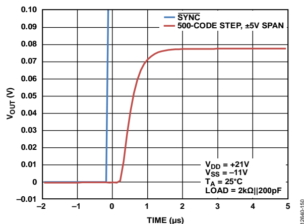
Figure 43. 500-Code Step Settling Time, \pm 5 V Range
