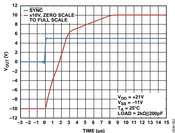
Figure 41. Full-Scale Settling Time (Rising Voltage Step), \pm 10 V Range
