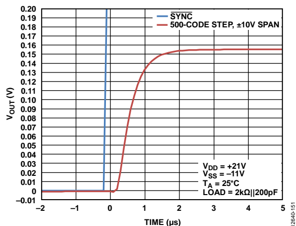
Figure 44. 500-Code Step Settling Time, \pm 10 V Range
