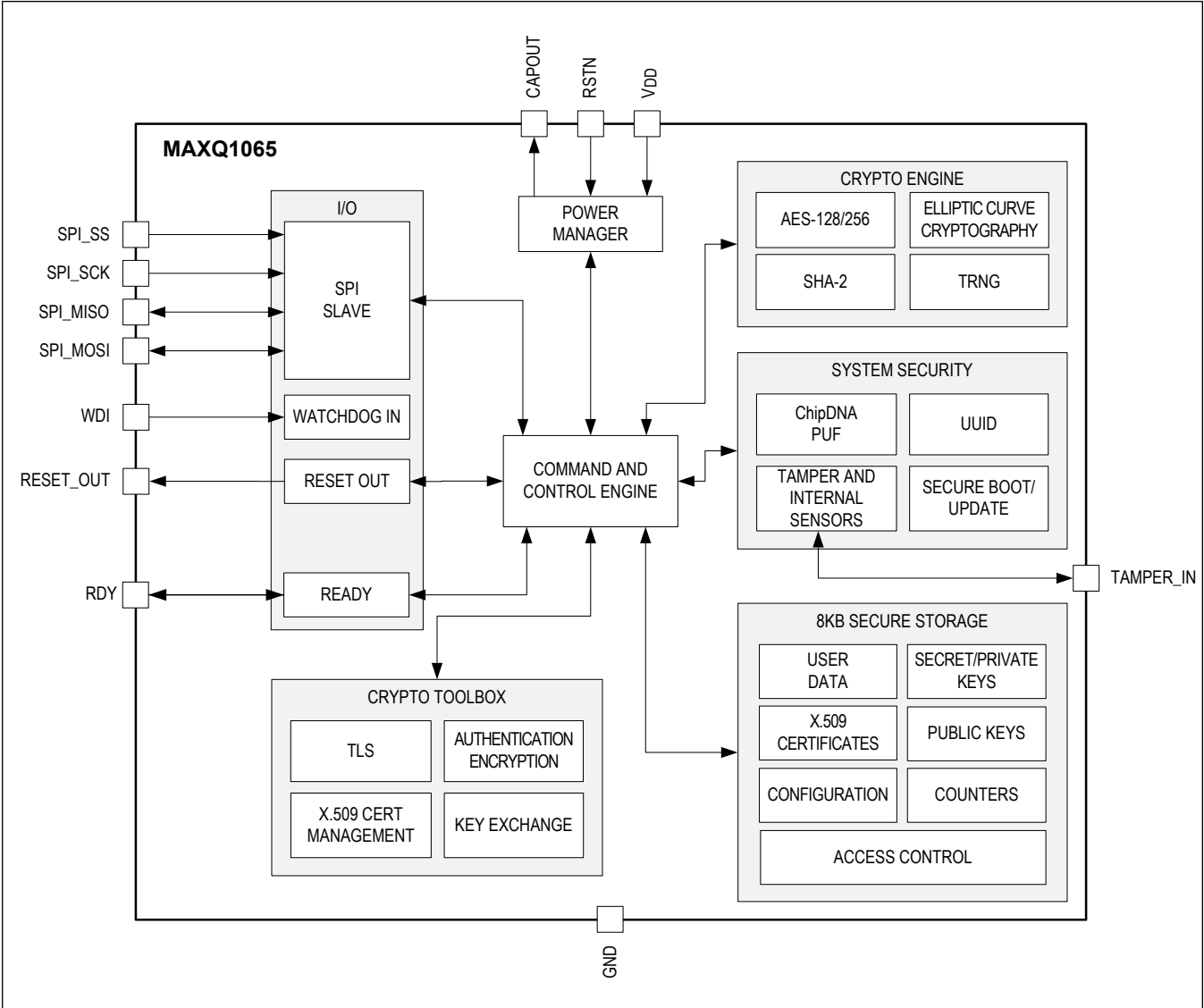
Block Diagram
