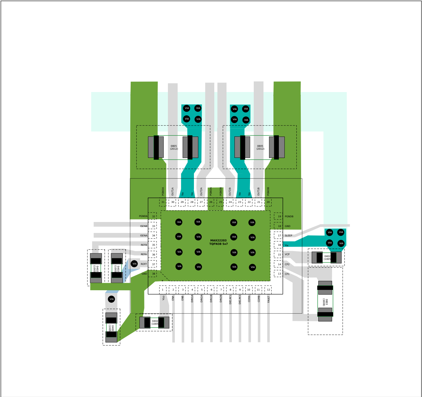
Figure 4. Recommended Layout
