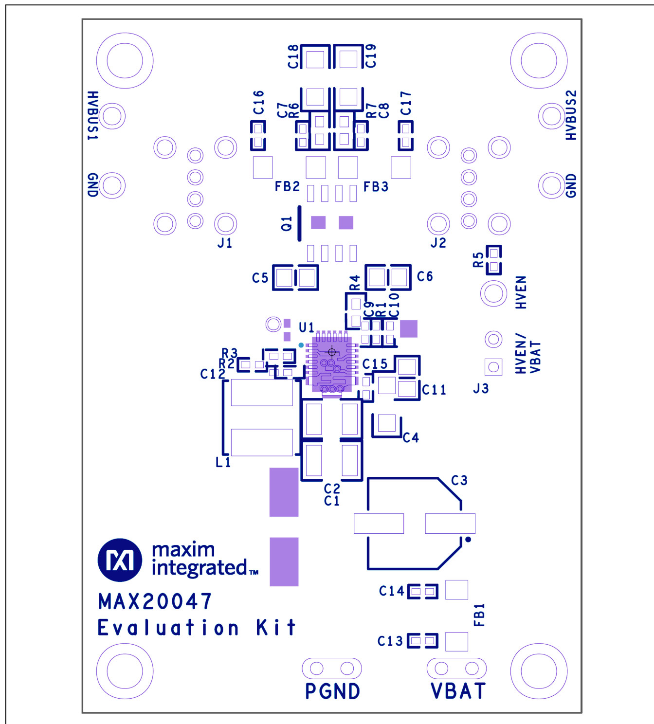
MAX20047 EV Kit Component Placement Guide—Top Silkscreen
