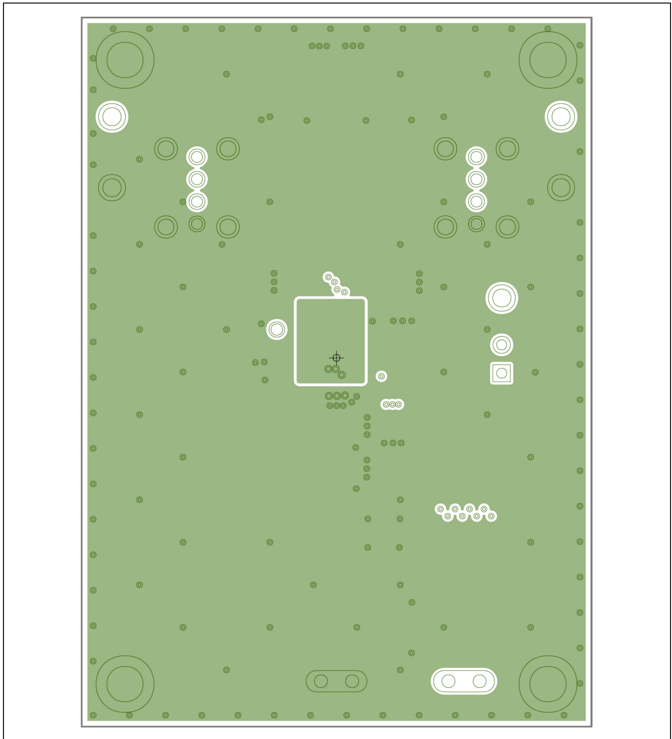
MAX20047 EV Kit PCB Layout—Layer 3
