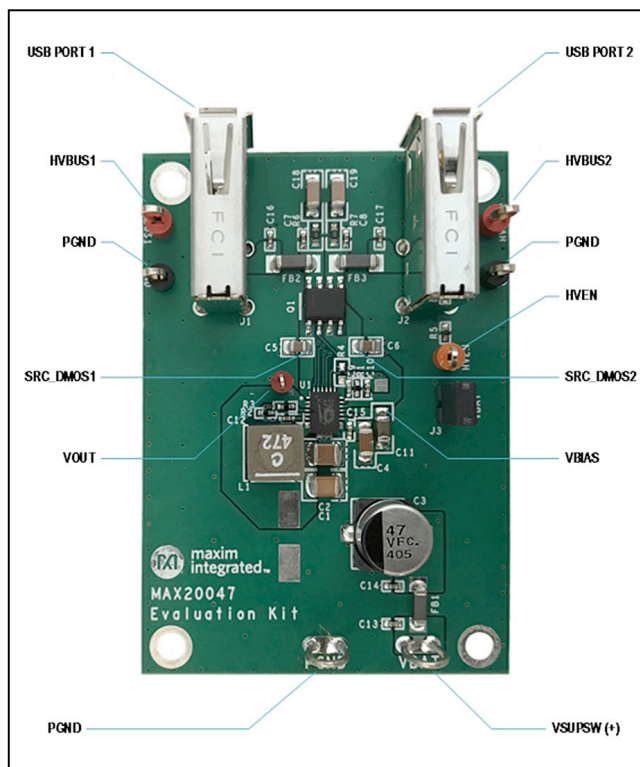
Figure 1. MAX20047 Evaluation Kit Test Points
