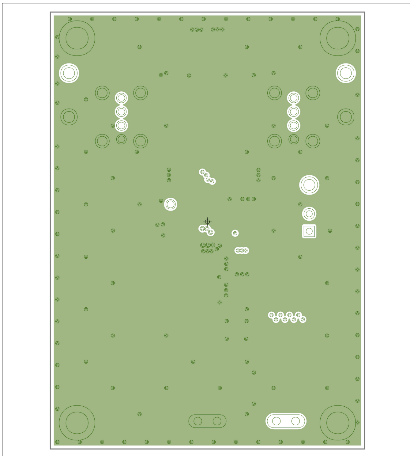
MAX20047 EV Kit PCB Layout—Layer 2
