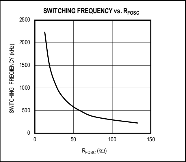
Figure 8. Frequency vs. R FOSC Resistance
