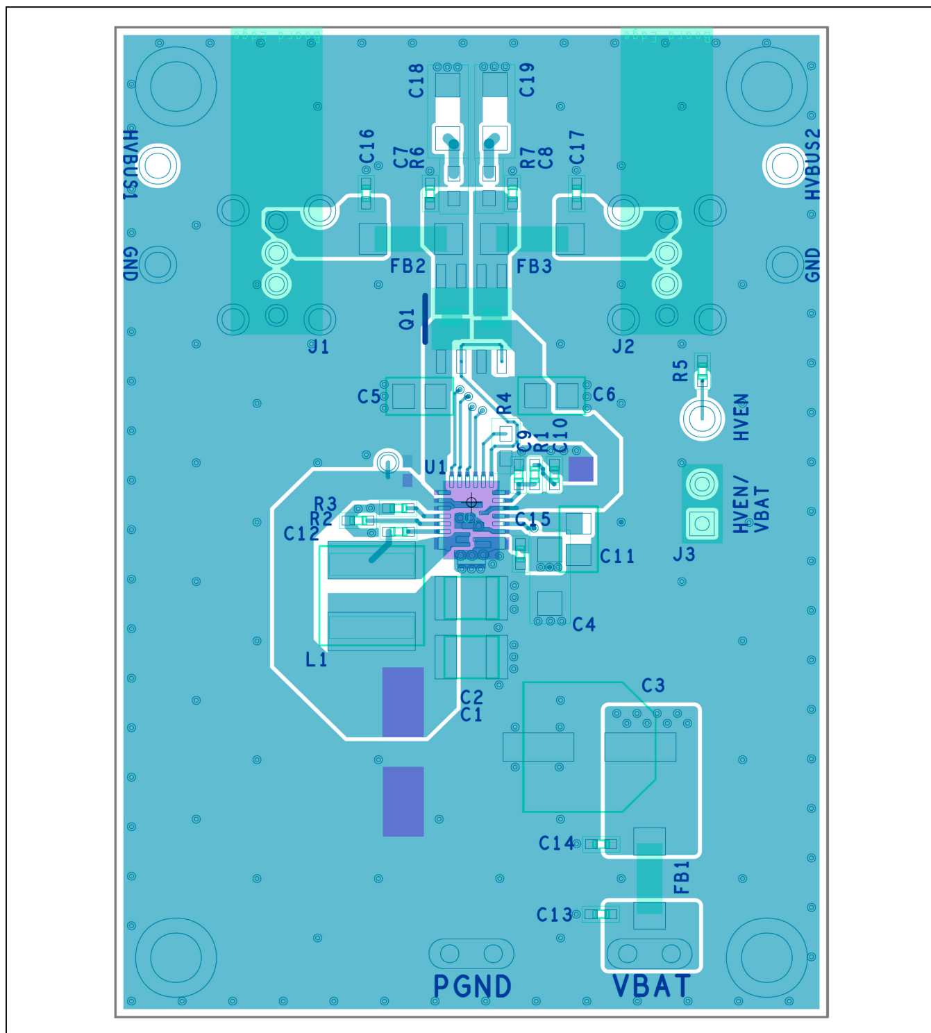
MAX20047 EV Kit PCB Layout—Top Layer
