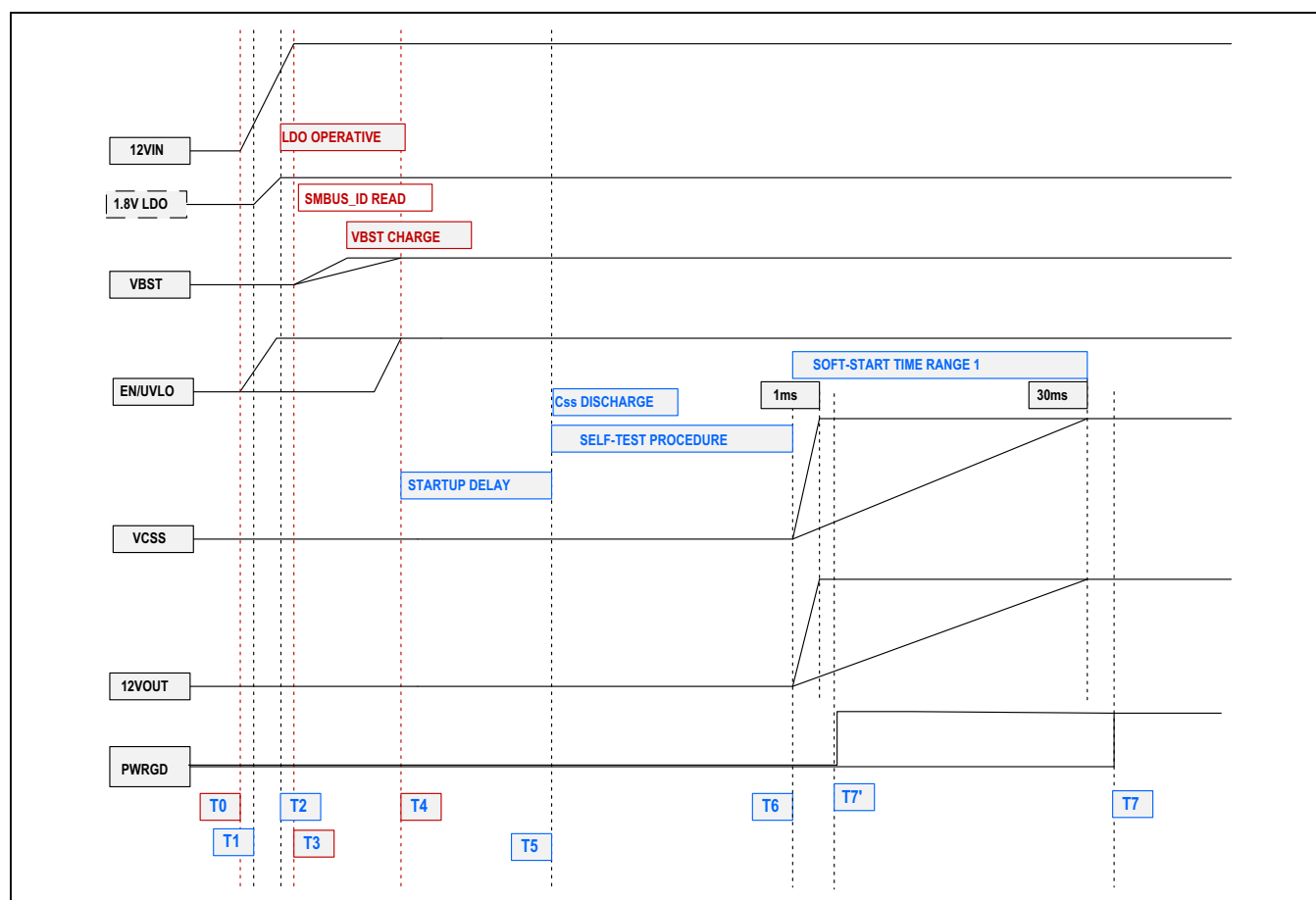
Figure 3. Startup Timing Diagram
