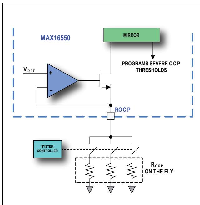
Figure 4. On-The-Fly Analog Programmable Moderate OCP Threshold (MAX16550)
