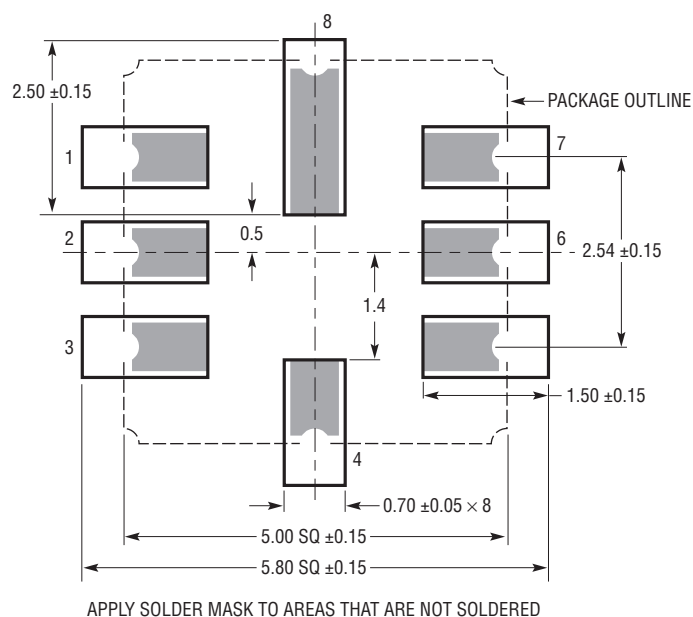
LS8 Package 8-Pin Leadless Chip Carrier (5mm × 5mm) (Reference LTC DWG # 05-08-1852 Rev B)
