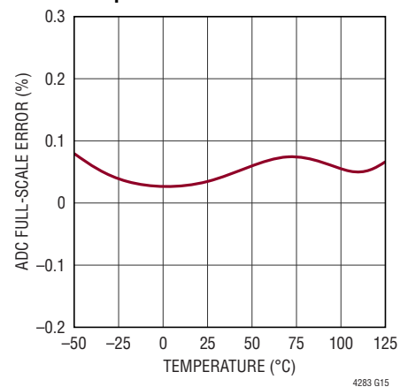
ADC Full-Scale Error vs Temperature
