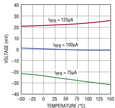
( R_{\text{FB}} - V_{\text{IN}} ) Voltage
