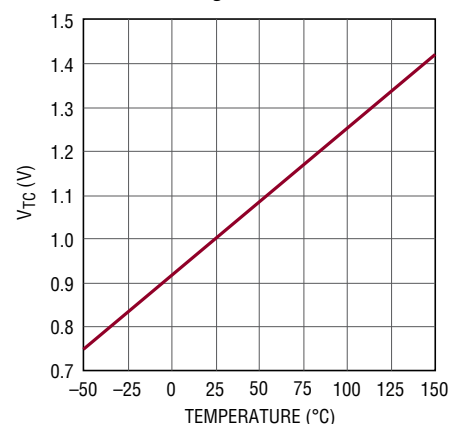
TC Pin Voltage
