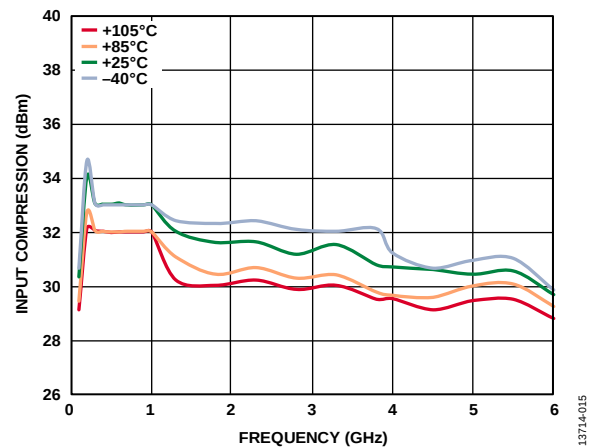
Figure 19. Input Compression 0.1 dB Point vs. Frequency for Various Temperatures, V_{DD} = 3.3\text{ V}
