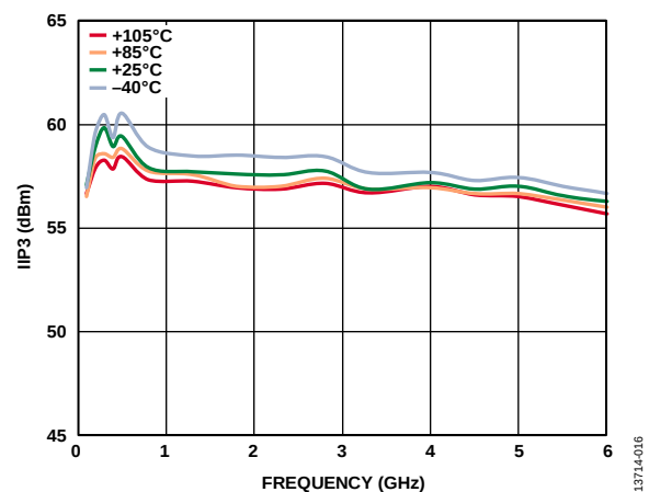
Figure 20. Input Third-Order Intercept (IIP3) Point vs. Frequency for Various Temperatures, V_{DD} = 3.3\text{ V}
