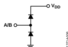
Figure 6. Logic Control (A/B) Interface Schematic
