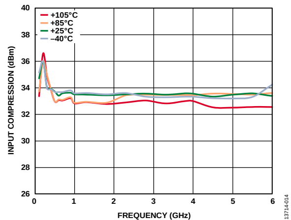
Figure 18. Input Compression 1 dB Point vs. Frequency for Various Temperatures, V_{DD} = 3.3\text{ V}
